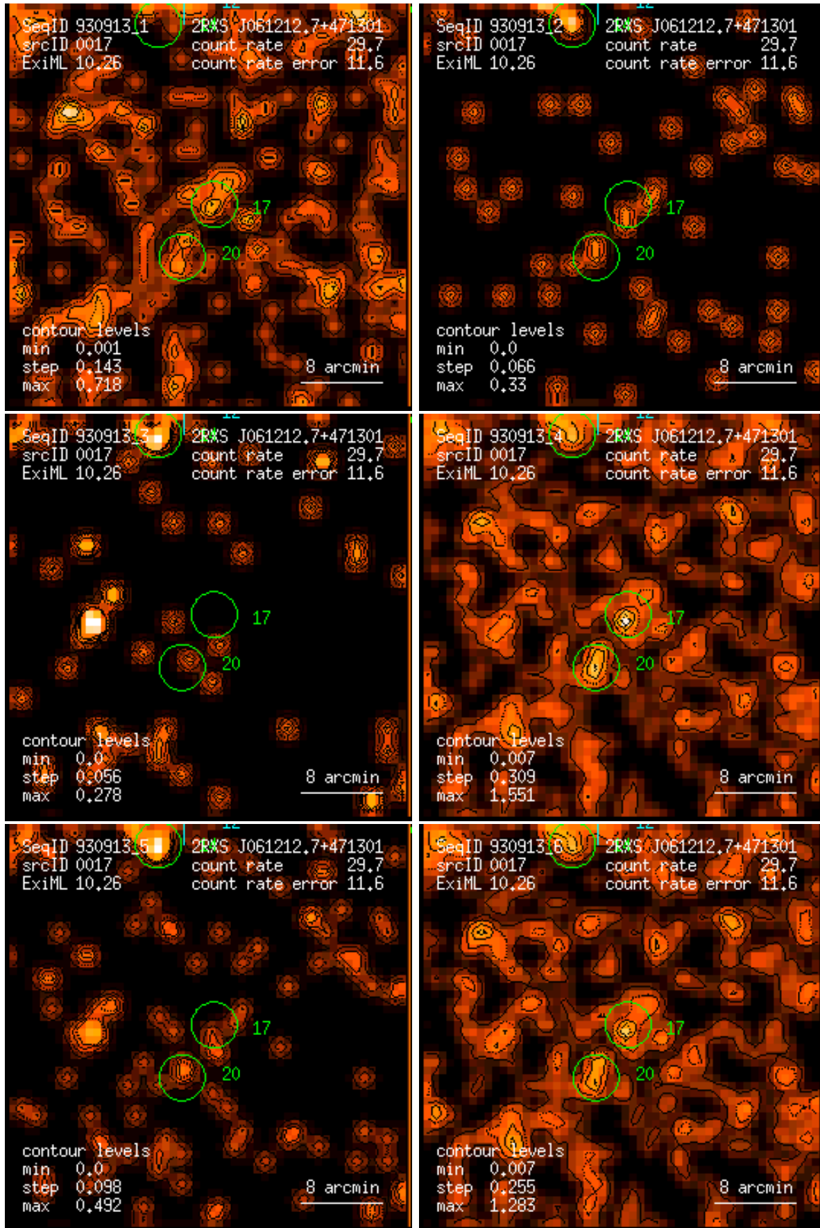
Figure 17: RASS 930913: detection 0017: band rate images, Gaussian filter: (1) PSPC channels 11 – 41, (2) 52 – 90, (3) 91 – 201, (4) 11 – 235, (5) 52 – 201, (6) 11 – 201. Broad band rates in counts/ks. Band rate contour levels in counts/ks/arcmin 2 .
