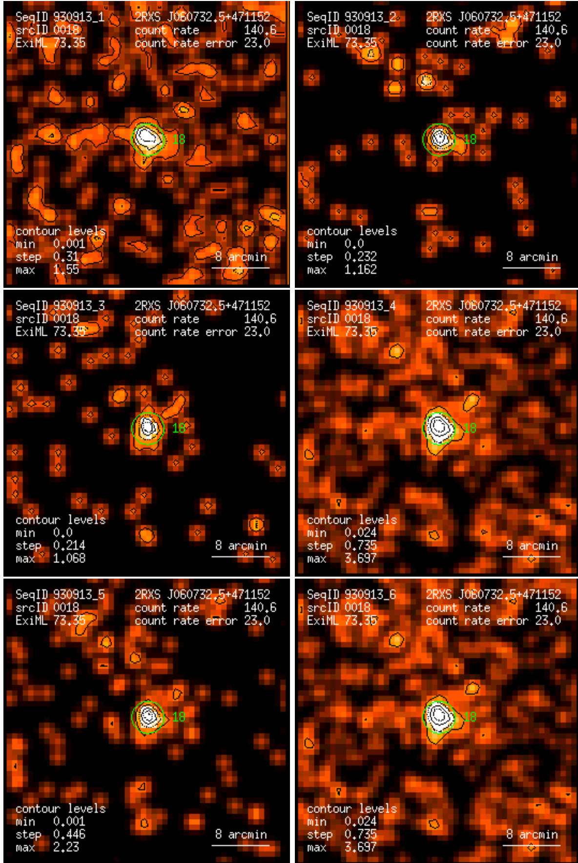
Figure 18: RASS 930913: detection 0018: band rate images, Gaussian filter: (1) PSPC channels 11 – 41, (2) 52 – 90, (3) 91 – 201, (4) 11 – 235, (5) 52 – 201, (6) 11 – 201. Broad band rates in counts/ks. Band rate contour levels in counts/ks/arcmin 2 .
