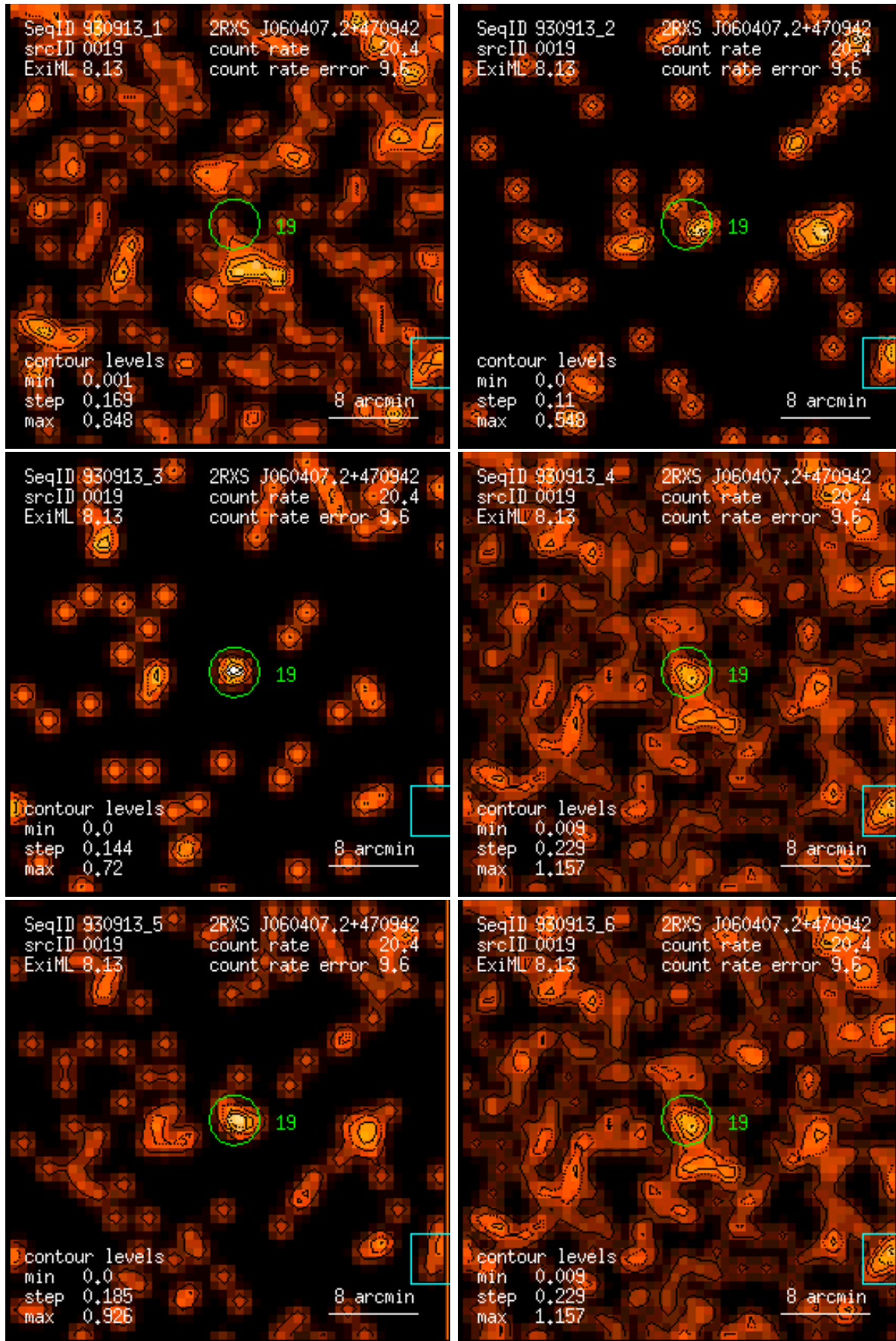
Figure 19: RASS 930913: detection 0019: band rate images, Gaussian filter: (1) PSPC channels 11 – 41, (2) 52 – 90, (3) 91 – 201, (4) 11 – 235, (5) 52 – 201, (6) 11 – 201. Broad band rates in counts/ks. Band rate contour levels in counts/ks/arcmin 2 .
