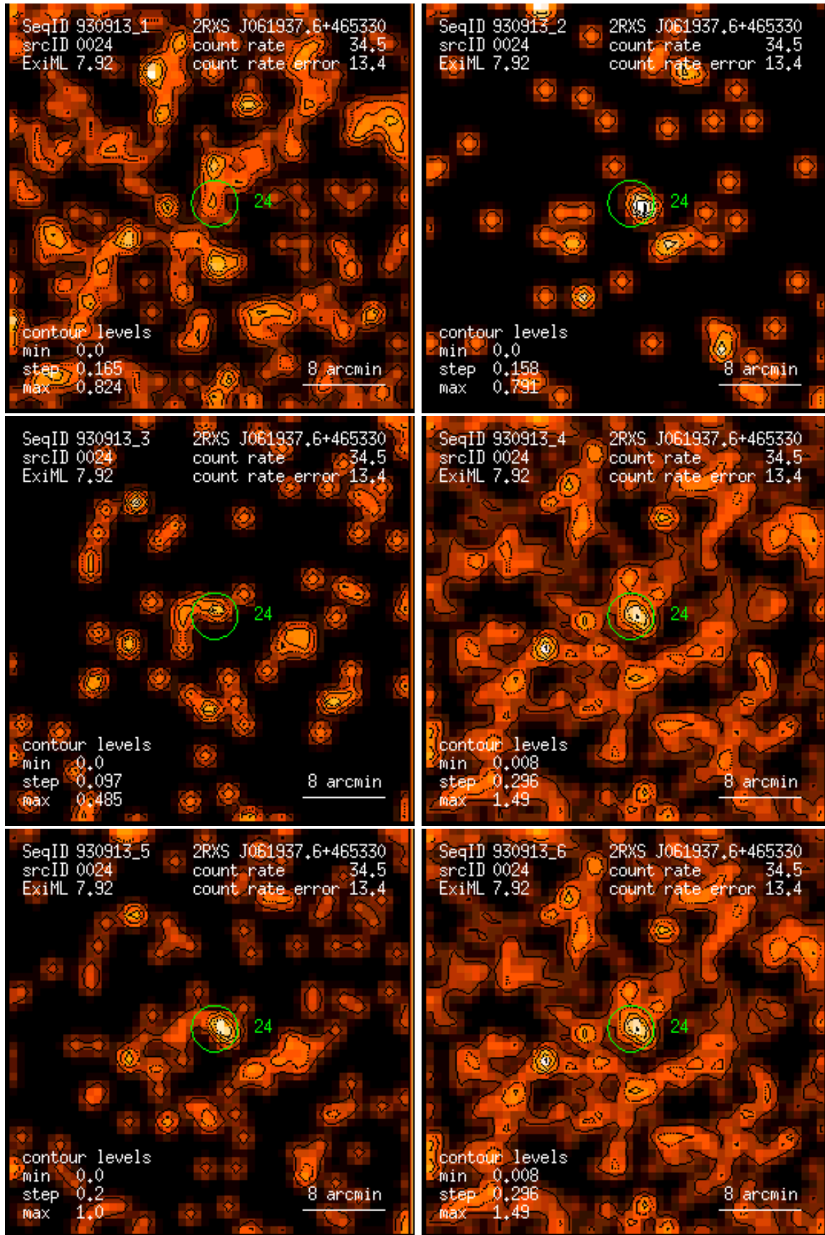
Figure 24: RASS 930913: detection 0024: band rate images, Gaussian filter: (1) PSPC channels 11 – 41, (2) 52 – 90, (3) 91 – 201, (4) 11 – 235, (5) 52 – 201, (6) 11 – 201. Broad band rates in counts/ks. Band rate contour levels in counts/ks/arcmin 2 .
