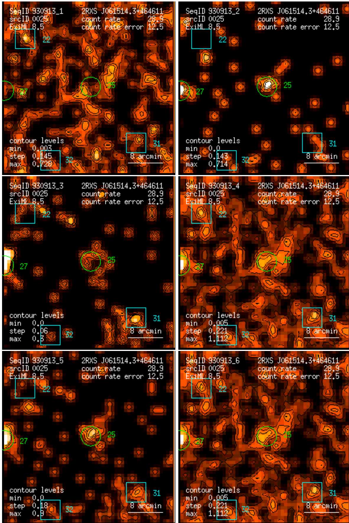
Figure 25: RASS 930913: detection 0025: band rate images, Gaussian filter: (1) PSPC channels 11 – 41, (2) 52 – 90, (3) 91 – 201, (4) 11 – 235, (5) 52 – 201, (6) 11 – 201. Broad band rates in counts/ks. Band rate contour levels in counts/ks/arcmin 2 .
