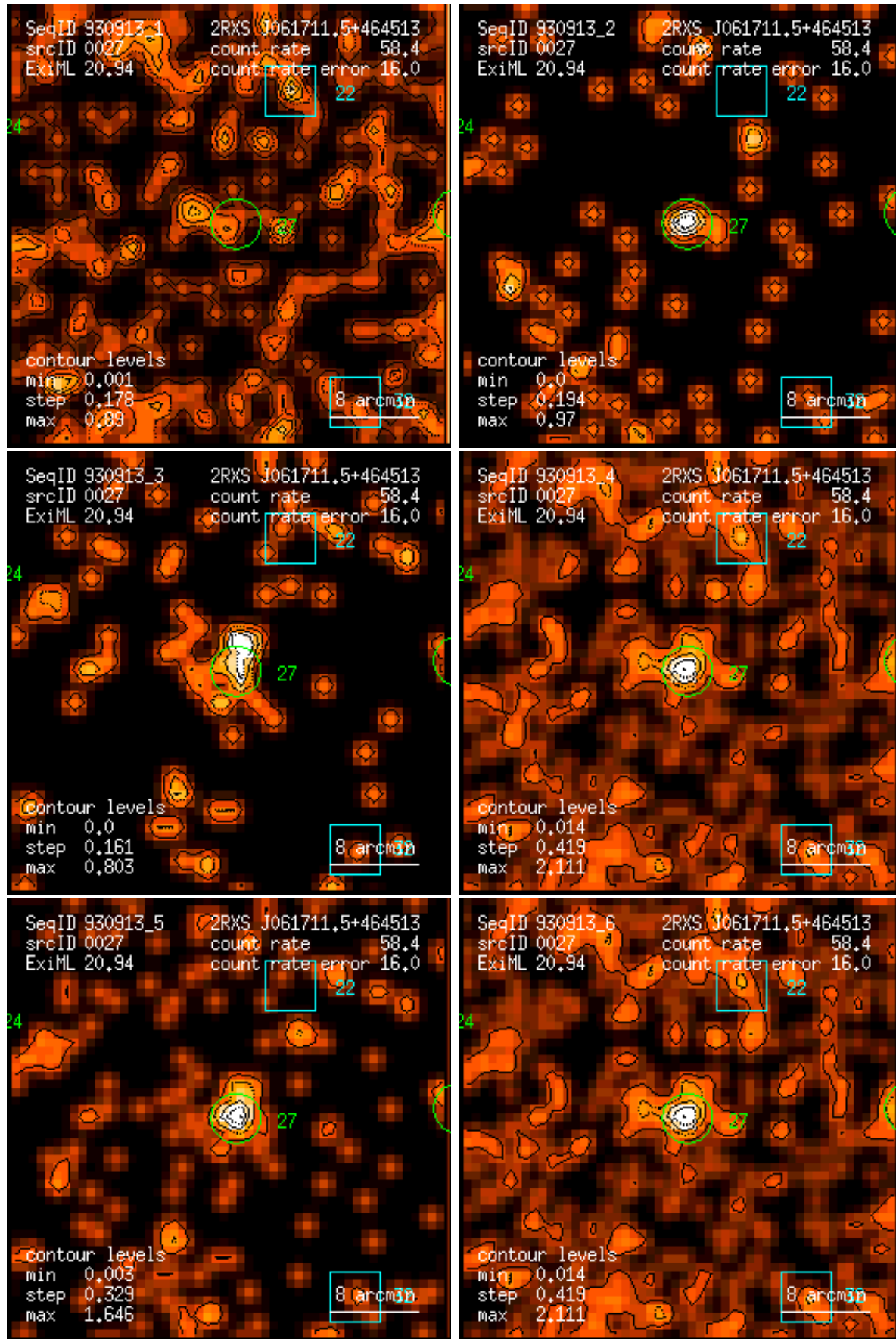
Figure 27: RASS 930913: detection 0027: band rate images, Gaussian filter: (1) PSPC channels 11 – 41, (2) 52 – 90, (3) 91 – 201, (4) 11 – 235, (5) 52 – 201, (6) 11 – 201. Broad band rates in counts/ks. Band rate contour levels in counts/ks/arcmin 2 .
