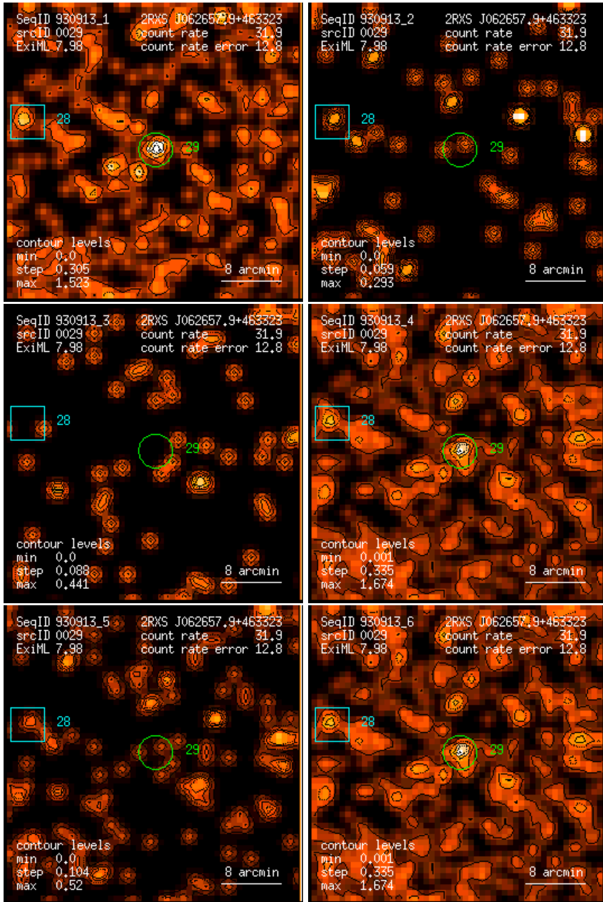
Figure 29: RASS 930913: detection 0029: band rate images, Gaussian filter: (1) PSPC channels 11 – 41, (2) 52 – 90, (3) 91 – 201, (4) 11 – 235, (5) 52 – 201, (6) 11 – 201. Broad band rates in counts/ks. Band rate contour levels in counts/ks/arcmin 2 .
