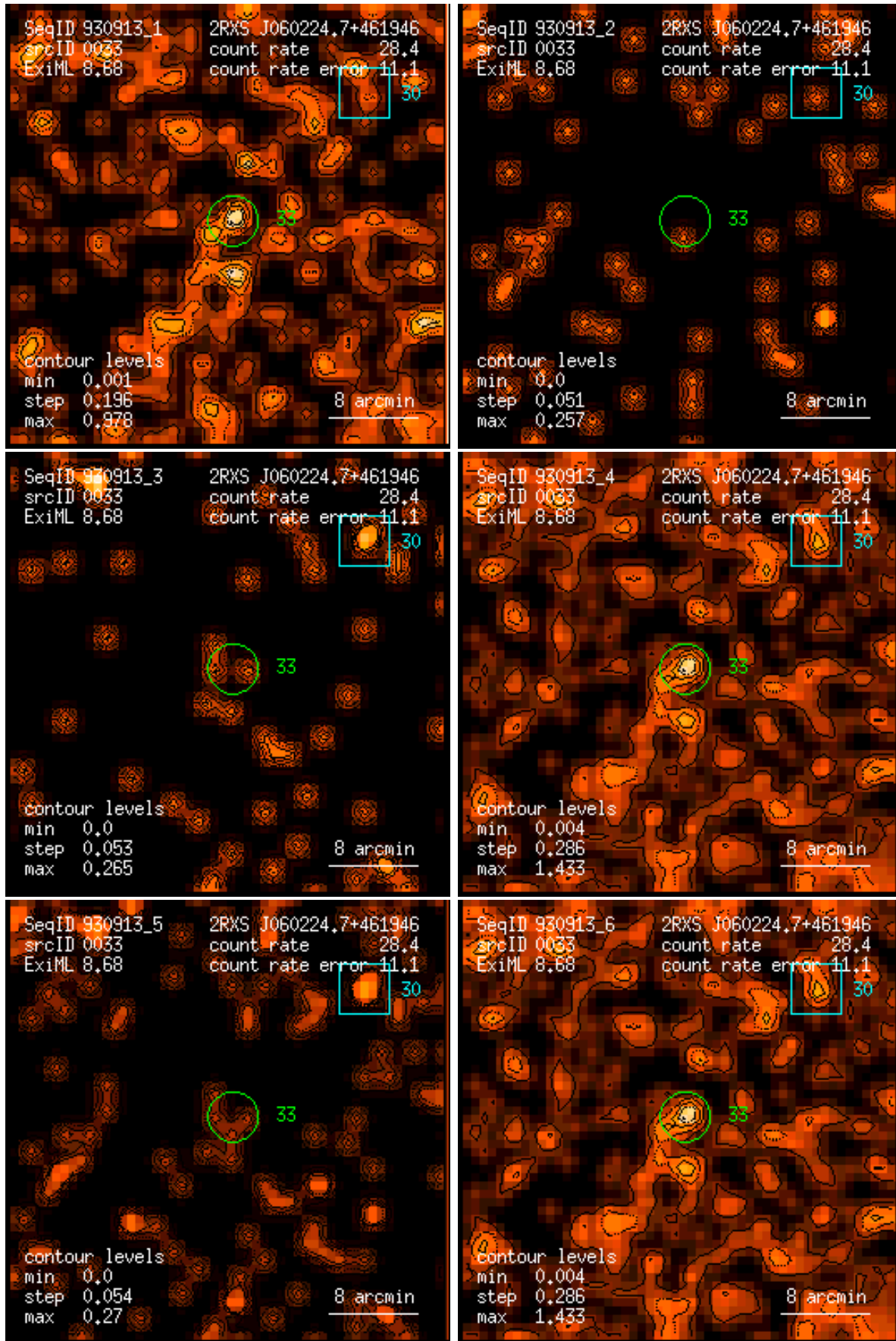
Figure 33: RASS 930913: detection 0033: band rate images, Gaussian filter: (1) PSPC channels 11 – 41, (2) 52 – 90, (3) 91 – 201, (4) 11 – 235, (5) 52 – 201, (6) 11 – 201. Broad band rates in counts/ks. Band rate contour levels in counts/ks/arcmin 2 .
