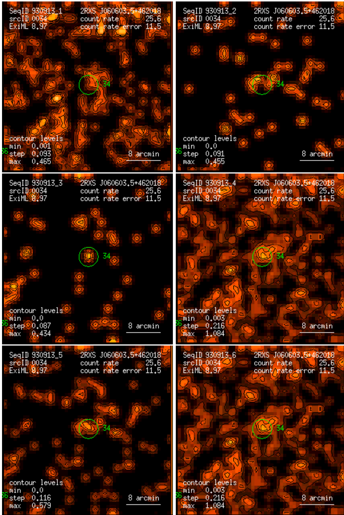
Figure 34: RASS 930913: detection 0034: band rate images, Gaussian filter: (1) PSPC channels 11 – 41, (2) 52 – 90, (3) 91 – 201, (4) 11 – 235, (5) 52 – 201, (6) 11 – 201. Broad band rates in counts/ks. Band rate contour levels in counts/ks/arcmin 2 .
