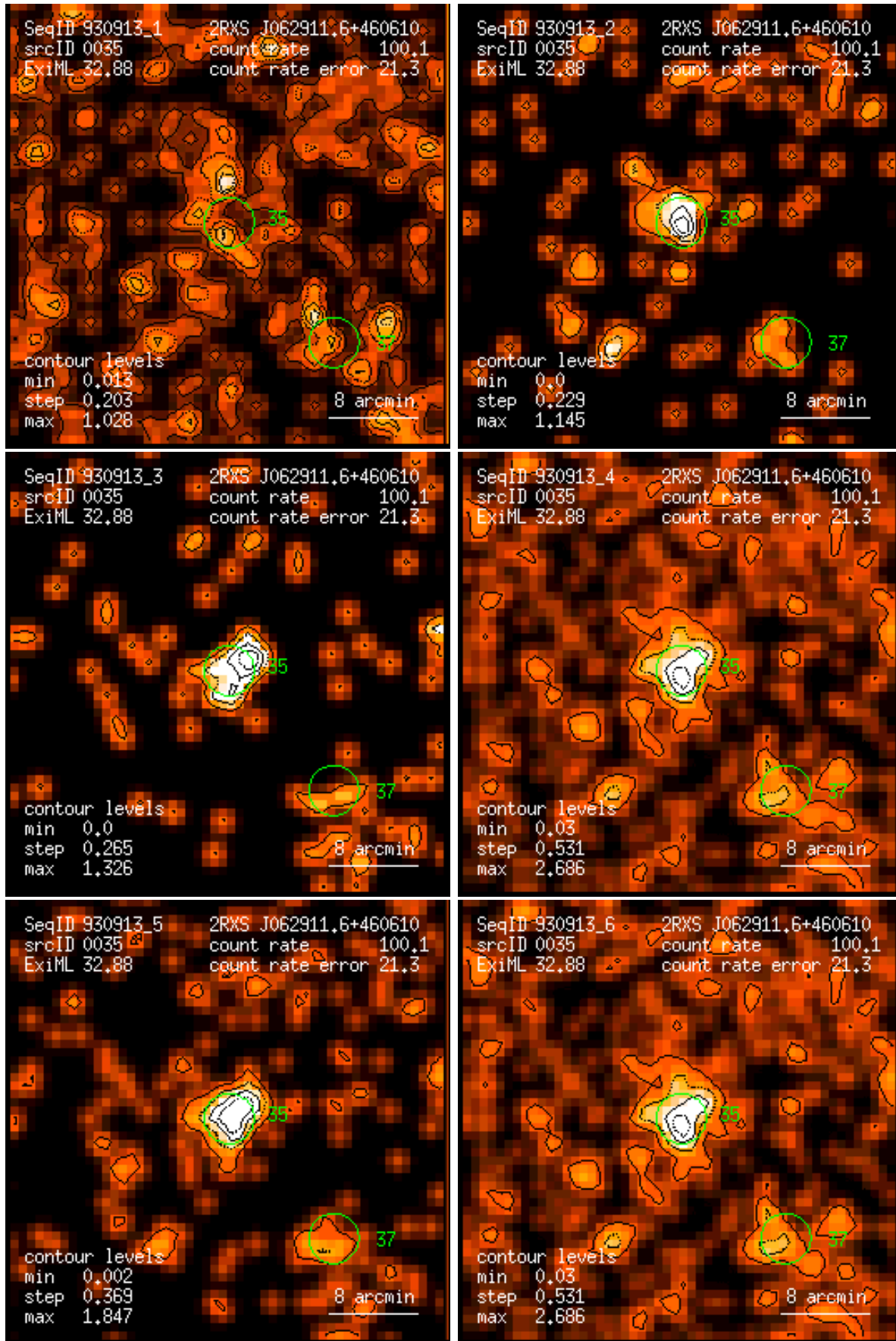
Figure 35: RASS 930913: detection 0035: band rate images, Gaussian filter: (1) PSPC channels 11 – 41, (2) 52 – 90, (3) 91 – 201, (4) 11 – 235, (5) 52 – 201, (6) 11 – 201. Broad band rates in counts/ks. Band rate contour levels in counts/ks/arcmin 2 .
