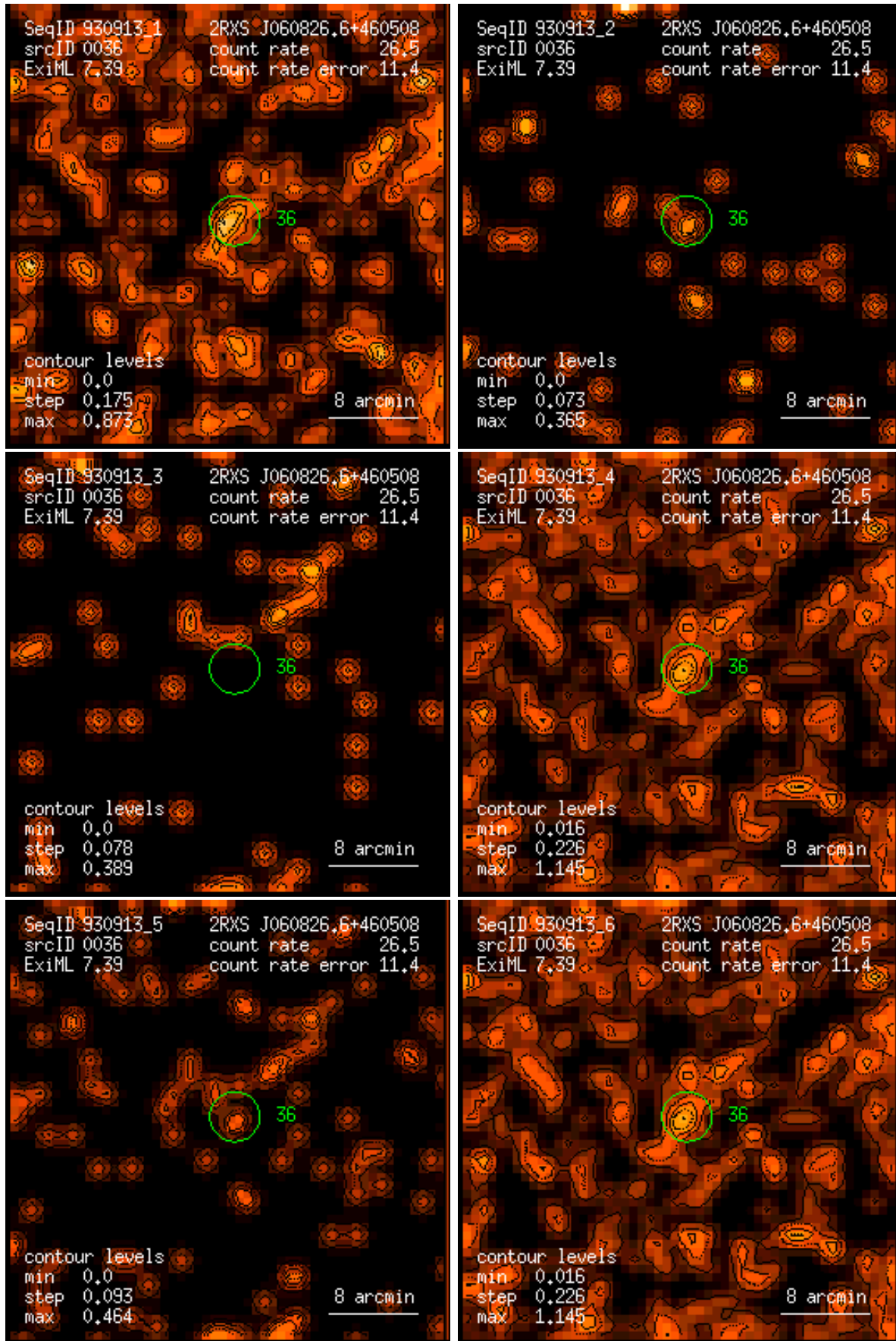
Figure 36: RASS 930913: detection 0036: band rate images, Gaussian filter: (1) PSPC channels 11 – 41, (2) 52 – 90, (3) 91 – 201, (4) 11 – 235, (5) 52 – 201, (6) 11 – 201. Broad band rates in counts/ks. Band rate contour levels in counts/ks/arcmin 2 .
