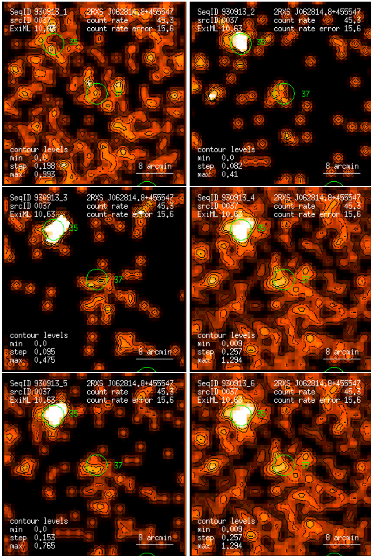
Figure 37: RASS 930913: detection 0037: band rate images, Gaussian filter: (1) PSPC channels 11 – 41, (2) 52 – 90, (3) 91 – 201, (4) 11 – 235, (5) 52 – 201, (6) 11 – 201. Broad band rates in counts/ks. Band rate contour levels in counts/ks/arcmin 2 .
