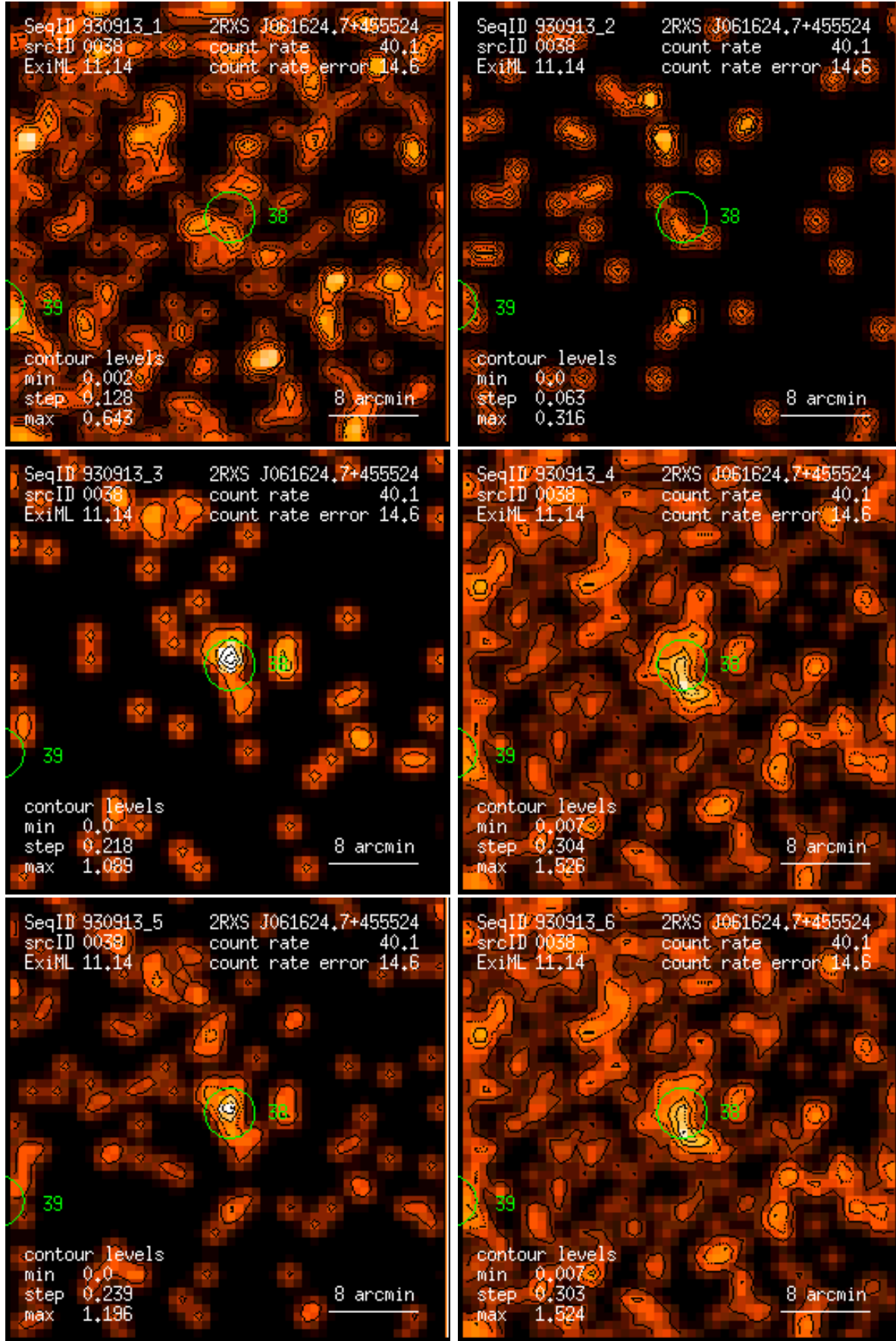
Figure 38: RASS 930913: detection 0038: band rate images, Gaussian filter: (1) PSPC channels 11 – 41, (2) 52 – 90, (3) 91 – 201, (4) 11 – 235, (5) 52 – 201, (6) 11 – 201. Broad band rates in counts/ks. Band rate contour levels in counts/ks/arcmin 2 .
