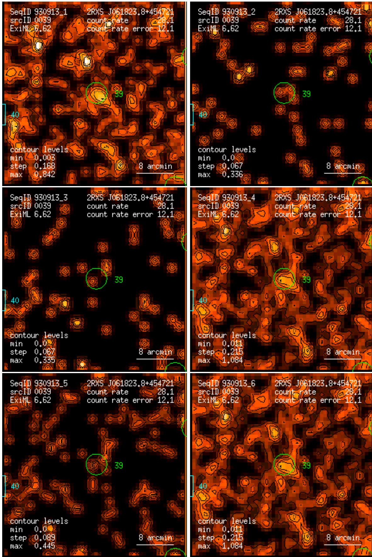
Figure 39: RASS 930913: detection 0039: band rate images, Gaussian filter: (1) PSPC channels 11 – 41, (2) 52 – 90, (3) 91 – 201, (4) 11 – 235, (5) 52 – 201, (6) 11 – 201. Broad band rates in counts/ks. Band rate contour levels in counts/ks/arcmin 2 .
