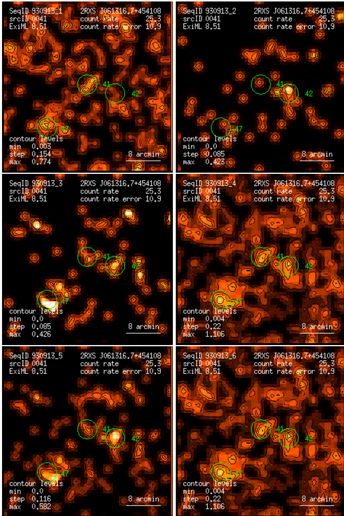
Figure 41: RASS 930913: detection 0041: band rate images, Gaussian filter: (1) PSPC channels 11 – 41, (2) 52 – 90, (3) 91 – 201, (4) 11 – 235, (5) 52 – 201, (6) 11 – 201. Broad band rates in counts/ks. Band rate contour levels in counts/ks/arcmin 2 .
