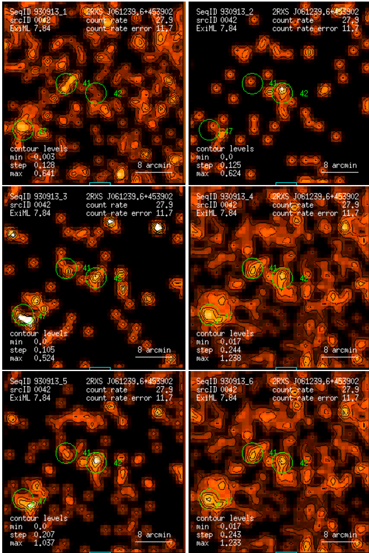
Figure 42: RASS 930913: detection 0042: band rate images, Gaussian filter: (1) PSPC channels 11 – 41, (2) 52 – 90, (3) 91 – 201, (4) 11 – 235, (5) 52 – 201, (6) 11 – 201. Broad band rates in counts/ks. Band rate contour levels in counts/ks/arcmin 2 .
