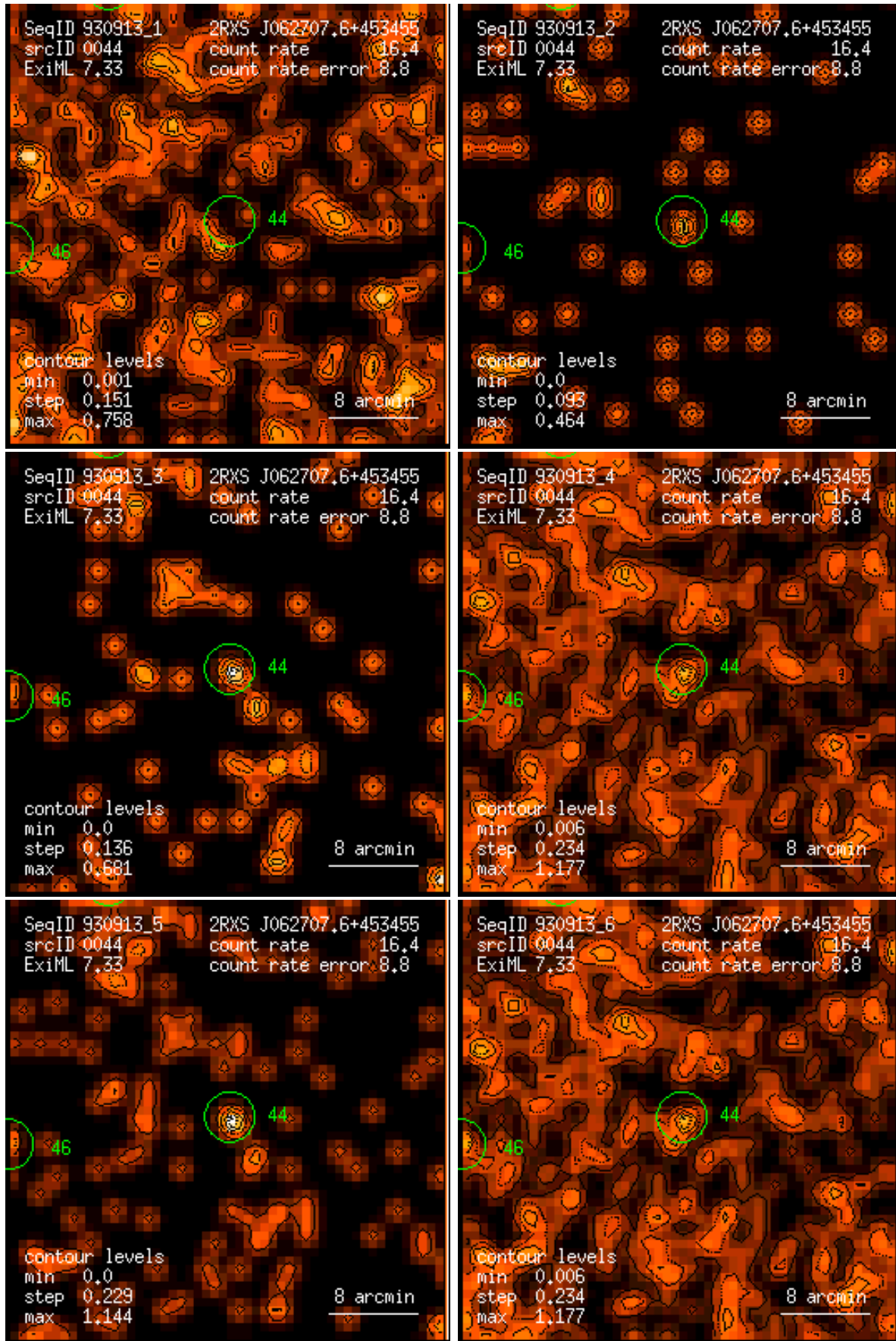
Figure 44: RASS 930913: detection 0044: band rate images, Gaussian filter: (1) PSPC channels 11 – 41, (2) 52 – 90, (3) 91 – 201, (4) 11 – 235, (5) 52 – 201, (6) 11 – 201. Broad band rates in counts/ks. Band rate contour levels in counts/ks/arcmin 2 .
