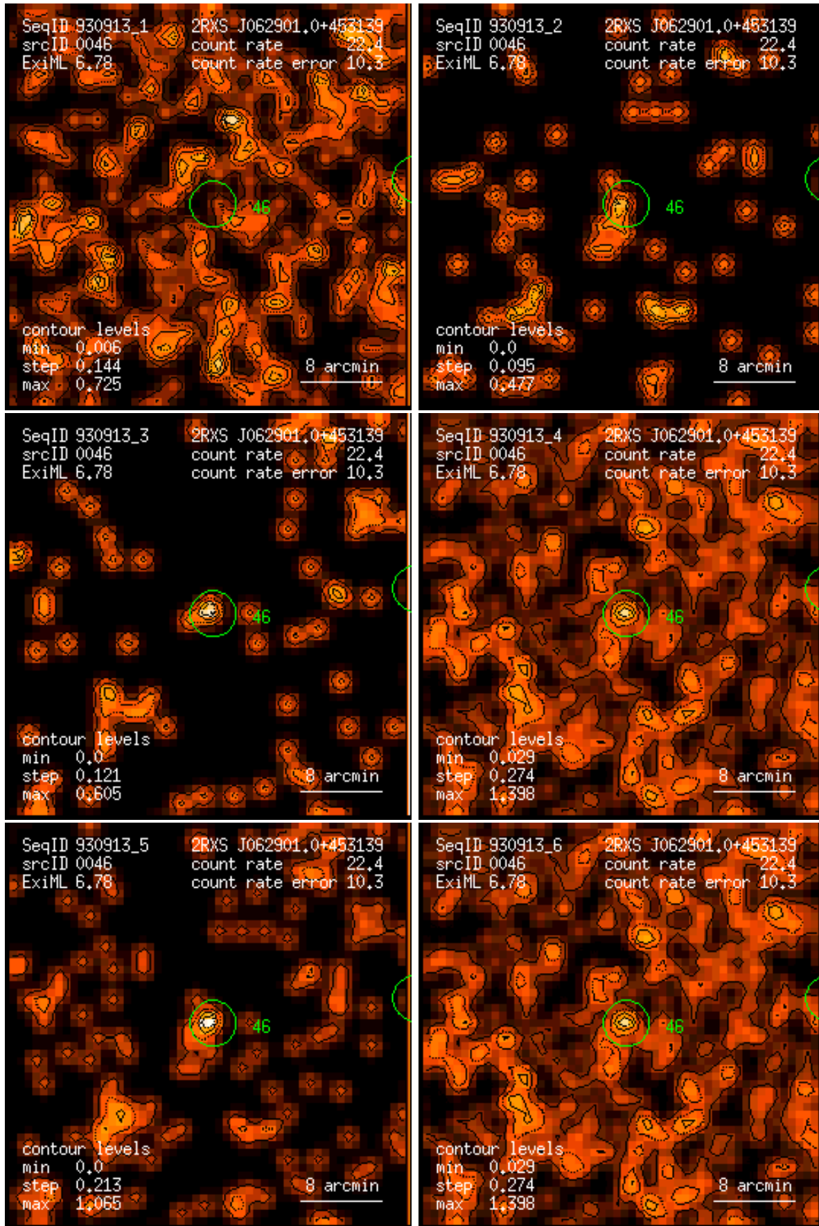
Figure 46: RASS 930913: detection 0046: band rate images, Gaussian filter: (1) PSPC channels 11 – 41, (2) 52 – 90, (3) 91 – 201, (4) 11 – 235, (5) 52 – 201, (6) 11 – 201. Broad band rates in counts/ks. Band rate contour levels in counts/ks/arcmin 2 .
