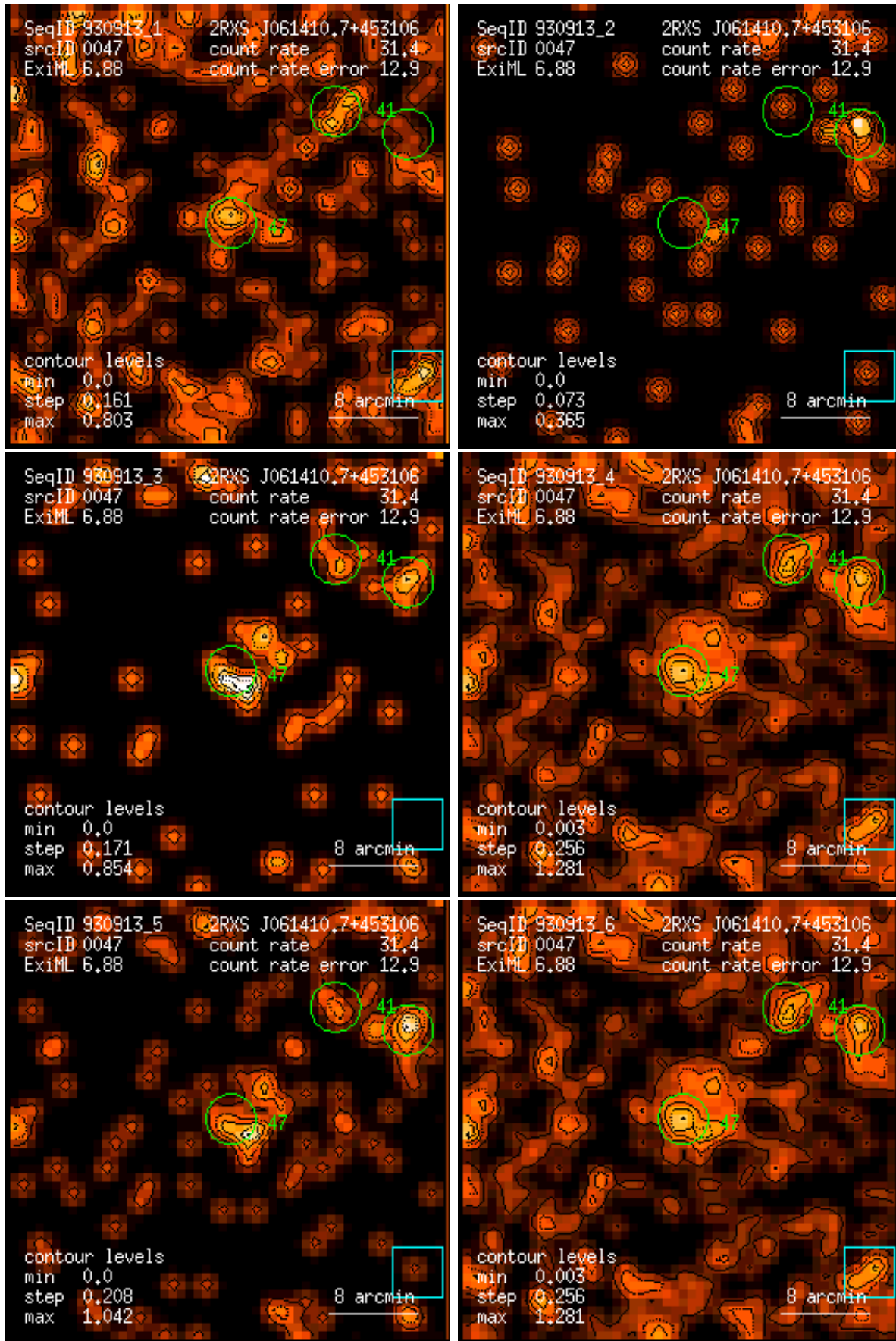
Figure 47: RASS 930913: detection 0047: band rate images, Gaussian filter: (1) PSPC channels 11 – 41, (2) 52 – 90, (3) 91 – 201, (4) 11 – 235, (5) 52 – 201, (6) 11 – 201. Broad band rates in counts/ks. Band rate contour levels in counts/ks/arcmin 2 .
