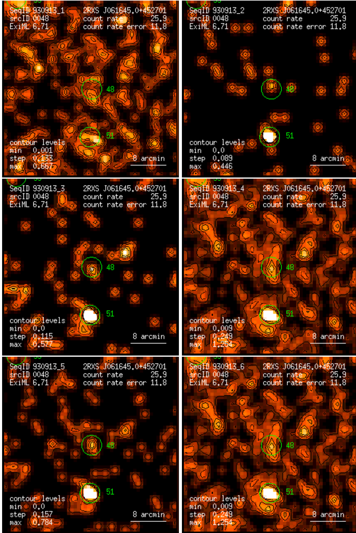
Figure 48: RASS 930913: detection 0048: band rate images, Gaussian filter: (1) PSPC channels 11 – 41, (2) 52 – 90, (3) 91 – 201, (4) 11 – 235, (5) 52 – 201, (6) 11 – 201. Broad band rates in counts/ks. Band rate contour levels in counts/ks/arcmin 2 .
