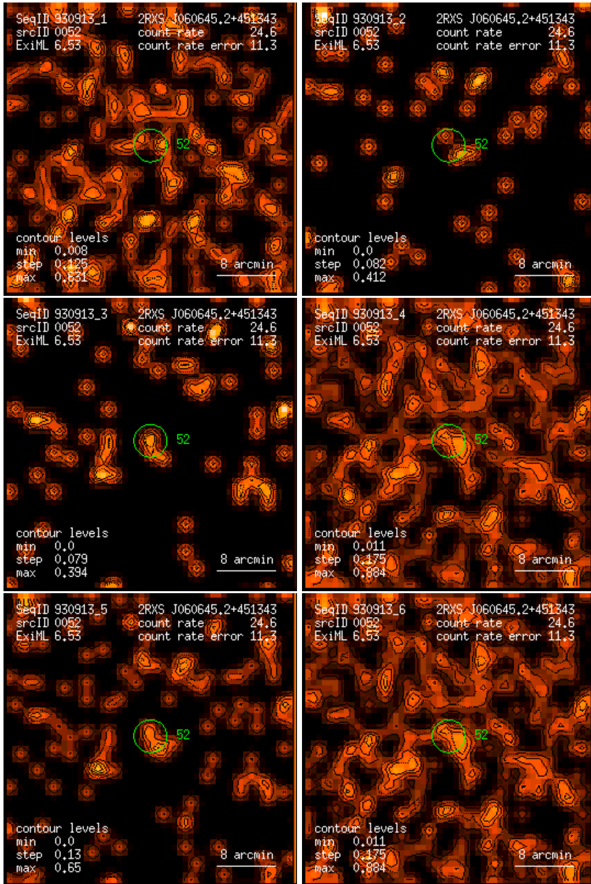
Figure 52: RASS 930913: detection 0052: band rate images, Gaussian filter: (1) PSPC channels 11 – 41, (2) 52 – 90, (3) 91 – 201, (4) 11 – 235, (5) 52 – 201, (6) 11 – 201. Broad band rates in counts/ks. Band rate contour levels in counts/ks/arcmin 2 .
