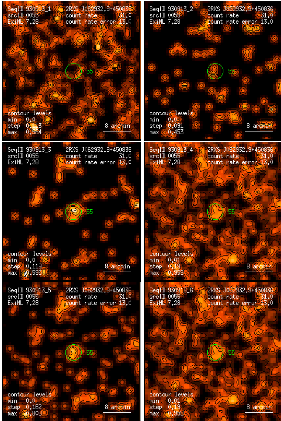
Figure 55: RASS 930913: detection 0055: band rate images, Gaussian filter: (1) PSPC channels 11 – 41, (2) 52 – 90, (3) 91 – 201, (4) 11 – 235, (5) 52 – 201, (6) 11 – 201. Broad band rates in counts/ks. Band rate contour levels in counts/ks/arcmin 2 .
