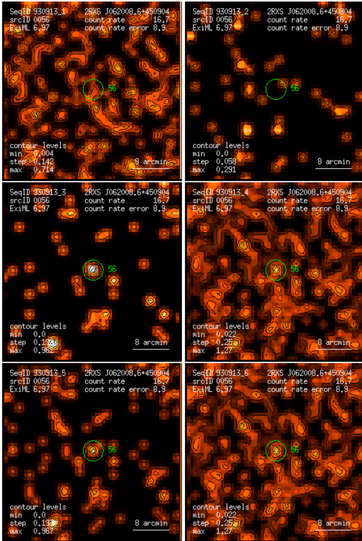
Figure 56: RASS 930913: detection 0056: band rate images, Gaussian filter: (1) PSPC channels 11 – 41, (2) 52 – 90, (3) 91 – 201, (4) 11 – 235, (5) 52 – 201, (6) 11 – 201. Broad band rates in counts/ks. Band rate contour levels in counts/ks/arcmin 2 .
