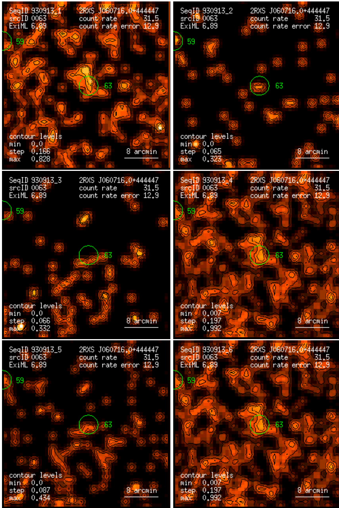
Figure 63: RASS 930913: detection 0063: band rate images, Gaussian filter: (1) PSPC channels 11 – 41, (2) 52 – 90, (3) 91 – 201, (4) 11 – 235, (5) 52 – 201, (6) 11 – 201. Broad band rates in counts/ks. Band rate contour levels in counts/ks/arcmin 2 .
