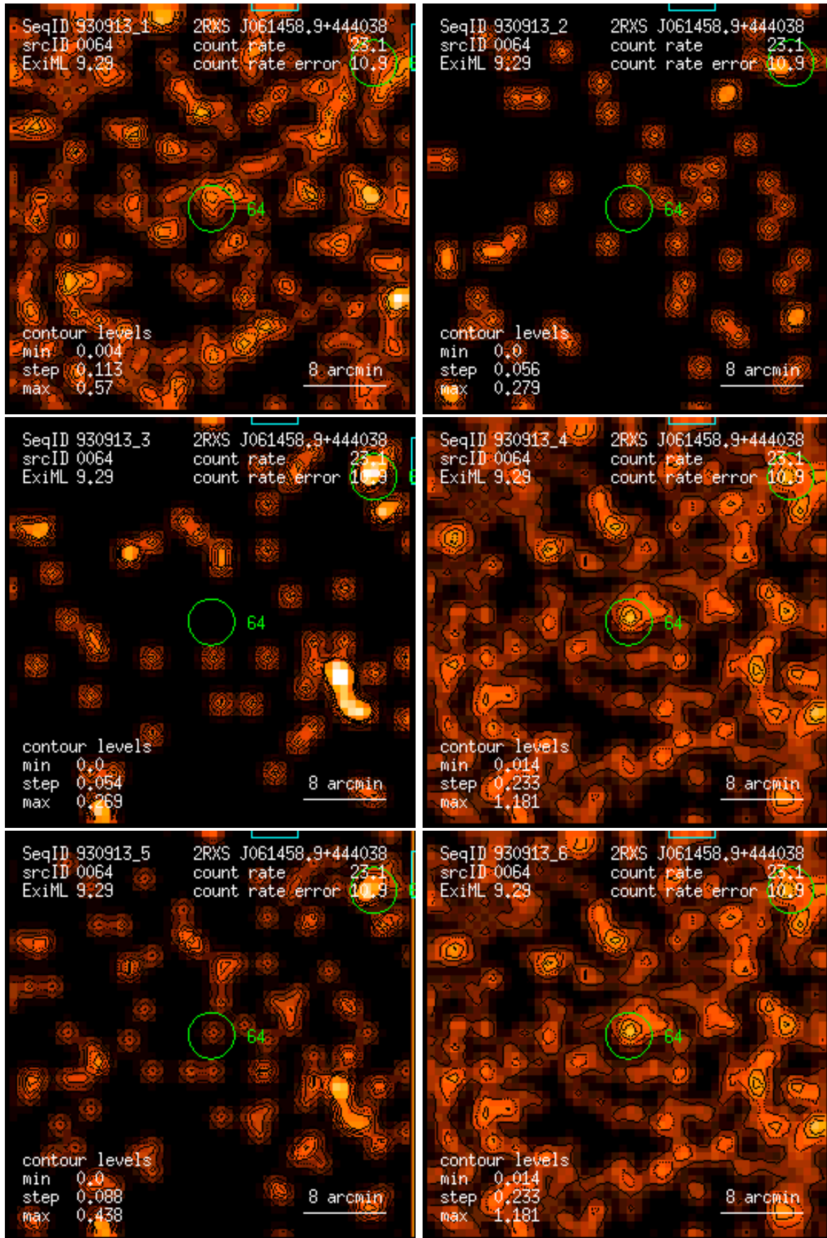
Figure 64: RASS 930913: detection 0064: band rate images, Gaussian filter: (1) PSPC channels 11 – 41, (2) 52 – 90, (3) 91 – 201, (4) 11 – 235, (5) 52 – 201, (6) 11 – 201. Broad band rates in counts/ks. Band rate contour levels in counts/ks/arcmin 2 .
