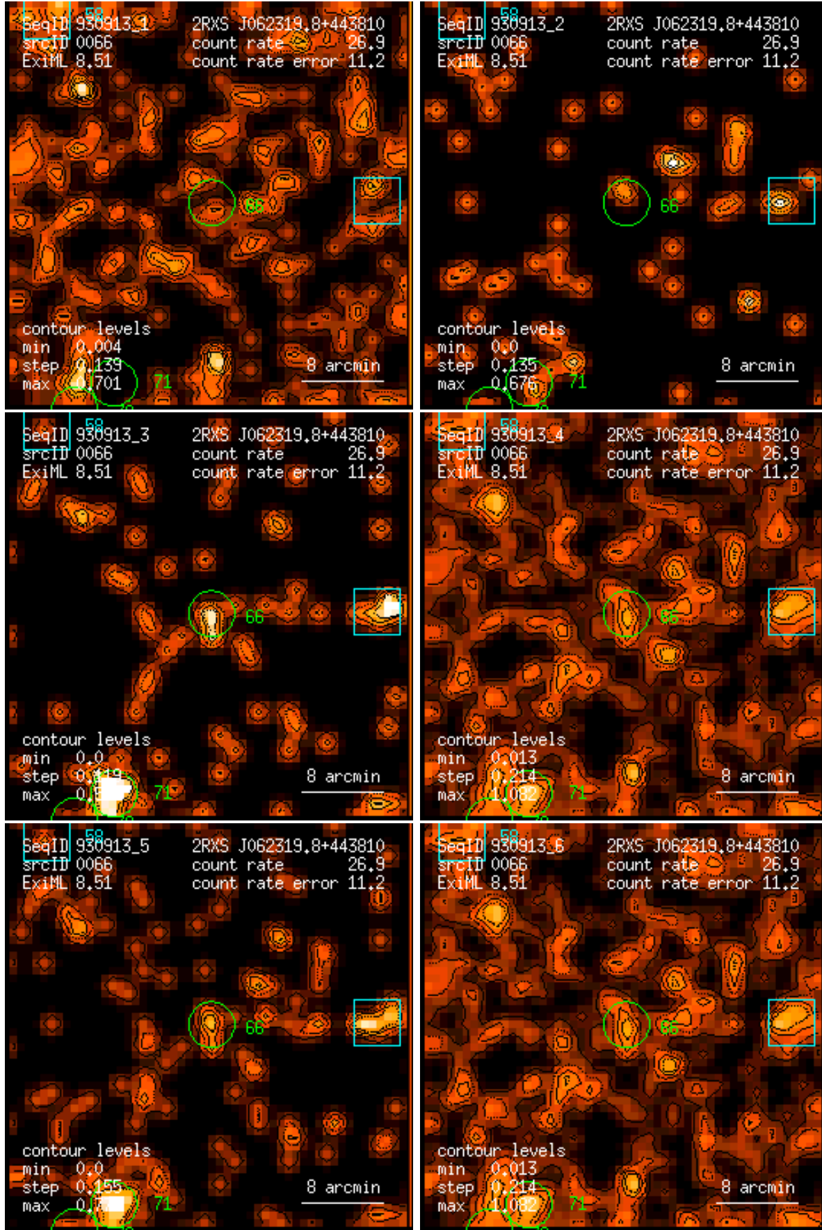
Figure 66: RASS 930913: detection 0066: band rate images, Gaussian filter: (1) PSPC channels 11 – 41, (2) 52 – 90, (3) 91 – 201, (4) 11 – 235, (5) 52 – 201, (6) 11 – 201. Broad band rates in counts/ks. Band rate contour levels in counts/ks/arcmin 2 .
