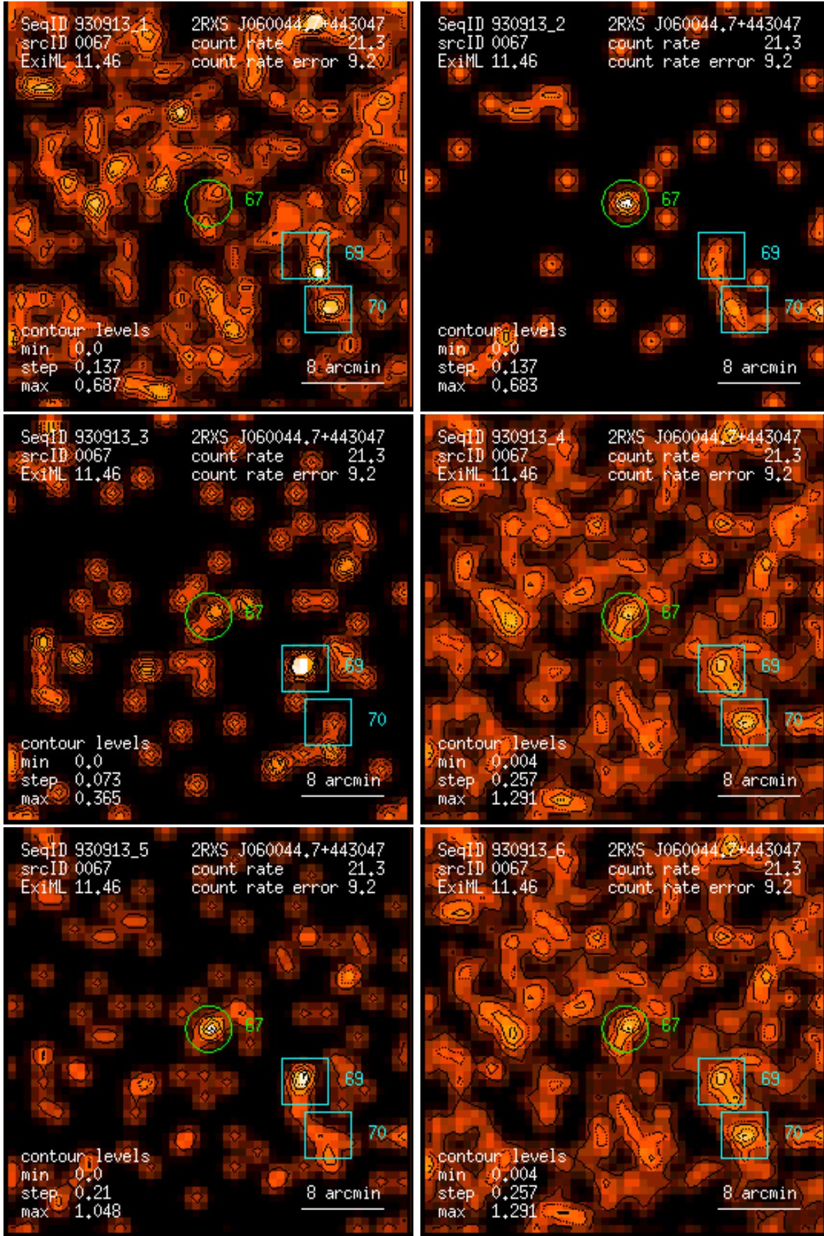
Figure 67: RASS 930913: detection 0067: band rate images, Gaussian filter: (1) PSPC channels 11 – 41, (2) 52 – 90, (3) 91 – 201, (4) 11 – 235, (5) 52 – 201, (6) 11 – 201. Broad band rates in counts/ks. Band rate contour levels in counts/ks/arcmin 2 .
