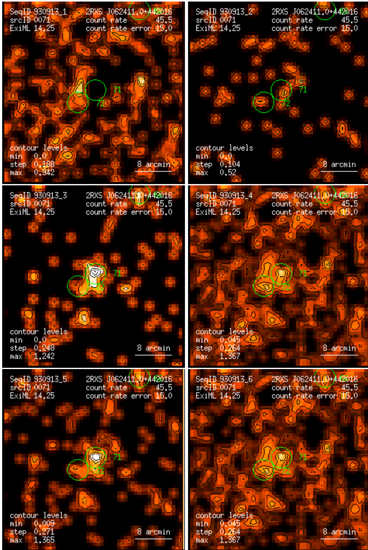
Figure 71: RASS 930913: detection 0071: band rate images, Gaussian filter: (1) PSPC channels 11 – 41, (2) 52 – 90, (3) 91 – 201, (4) 11 – 235, (5) 52 – 201, (6) 11 – 201. Broad band rates in counts/ks. Band rate contour levels in counts/ks/arcmin 2 .
