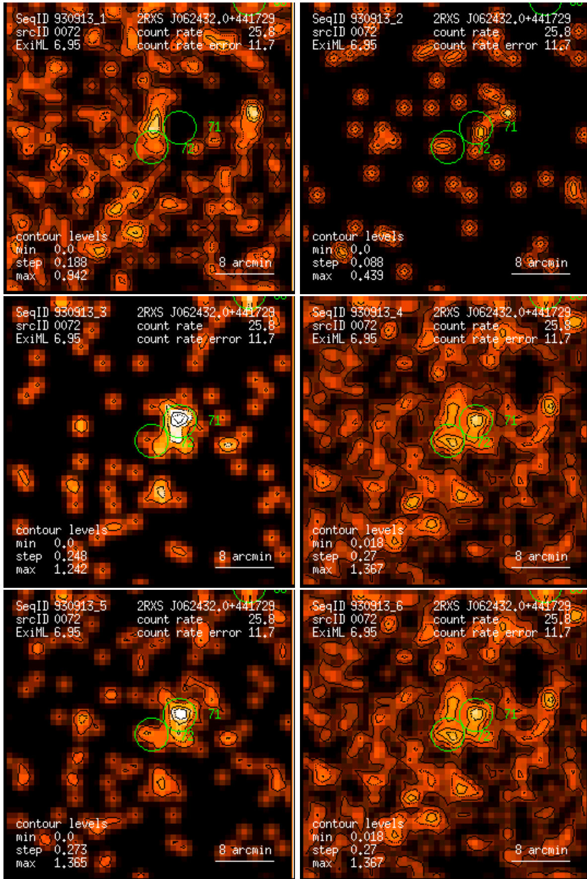
Figure 72: RASS 930913: detection 0072: band rate images, Gaussian filter: (1) PSPC channels 11 – 41, (2) 52 – 90, (3) 91 – 201, (4) 11 – 235, (5) 52 – 201, (6) 11 – 201. Broad band rates in counts/ks. Band rate contour levels in counts/ks/arcmin 2 .
