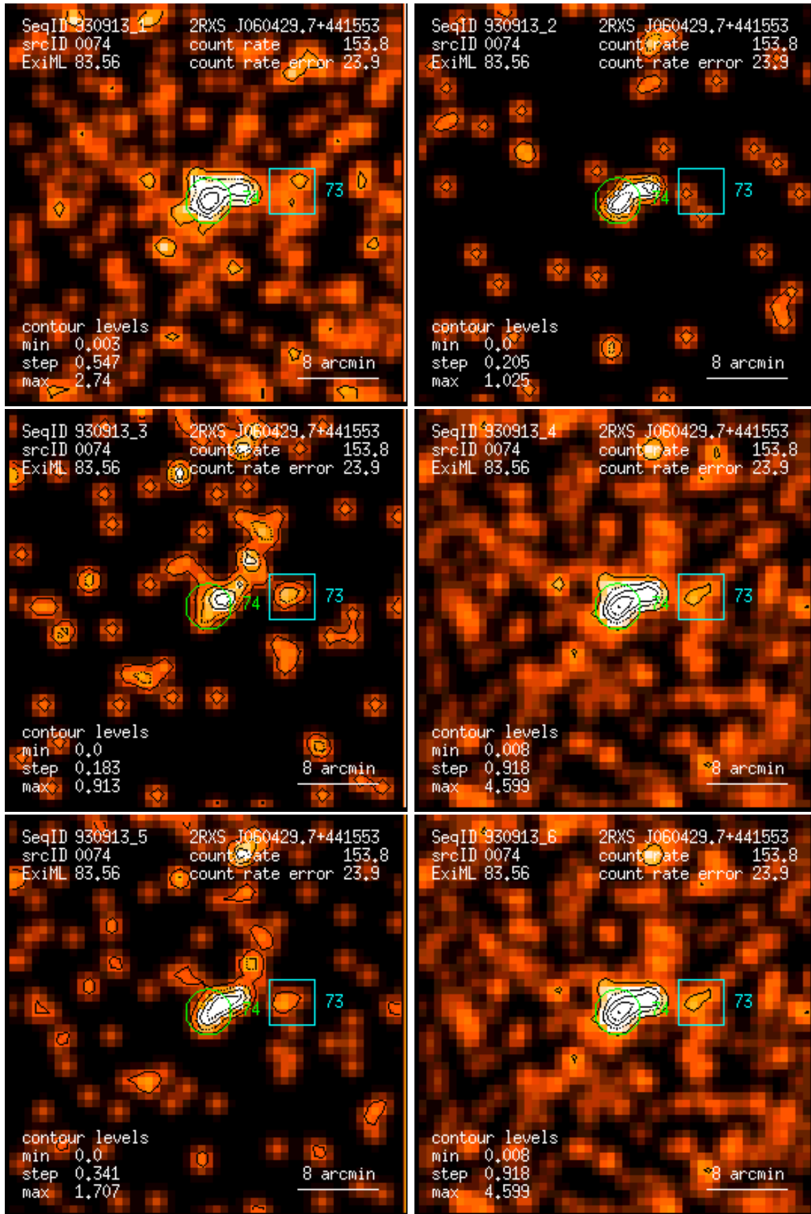
Figure 74: RASS 930913: detection 0074: band rate images, Gaussian filter: (1) PSPC channels 11 – 41, (2) 52 – 90, (3) 91 – 201, (4) 11 – 235, (5) 52 – 201, (6) 11 – 201. Broad band rates in counts/ks. Band rate contour levels in counts/ks/arcmin 2 .
