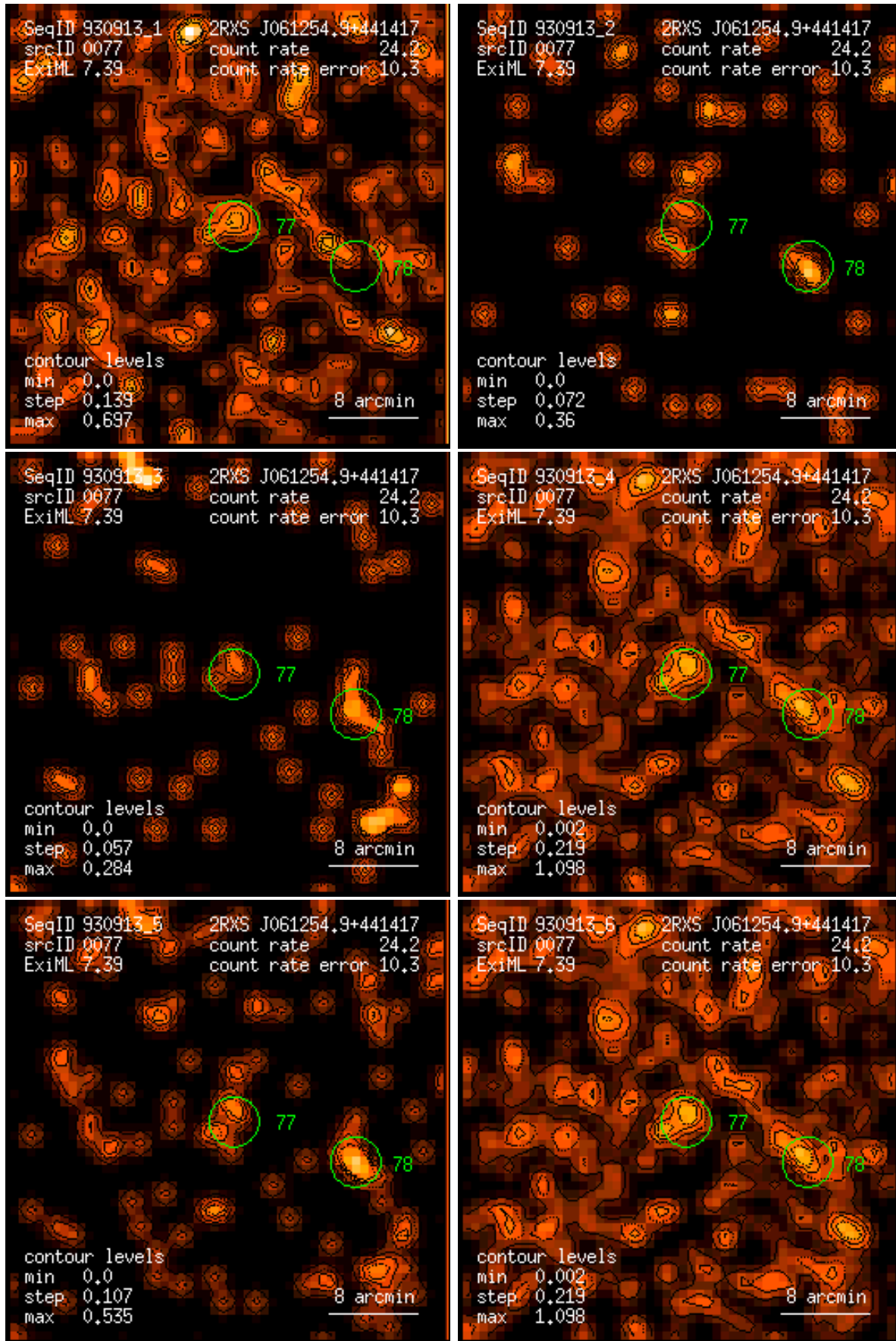
Figure 77: RASS 930913: detection 0077: band rate images, Gaussian filter: (1) PSPC channels 11 – 41, (2) 52 – 90, (3) 91 – 201, (4) 11 – 235, (5) 52 – 201, (6) 11 – 201. Broad band rates in counts/ks. Band rate contour levels in counts/ks/arcmin 2 .
