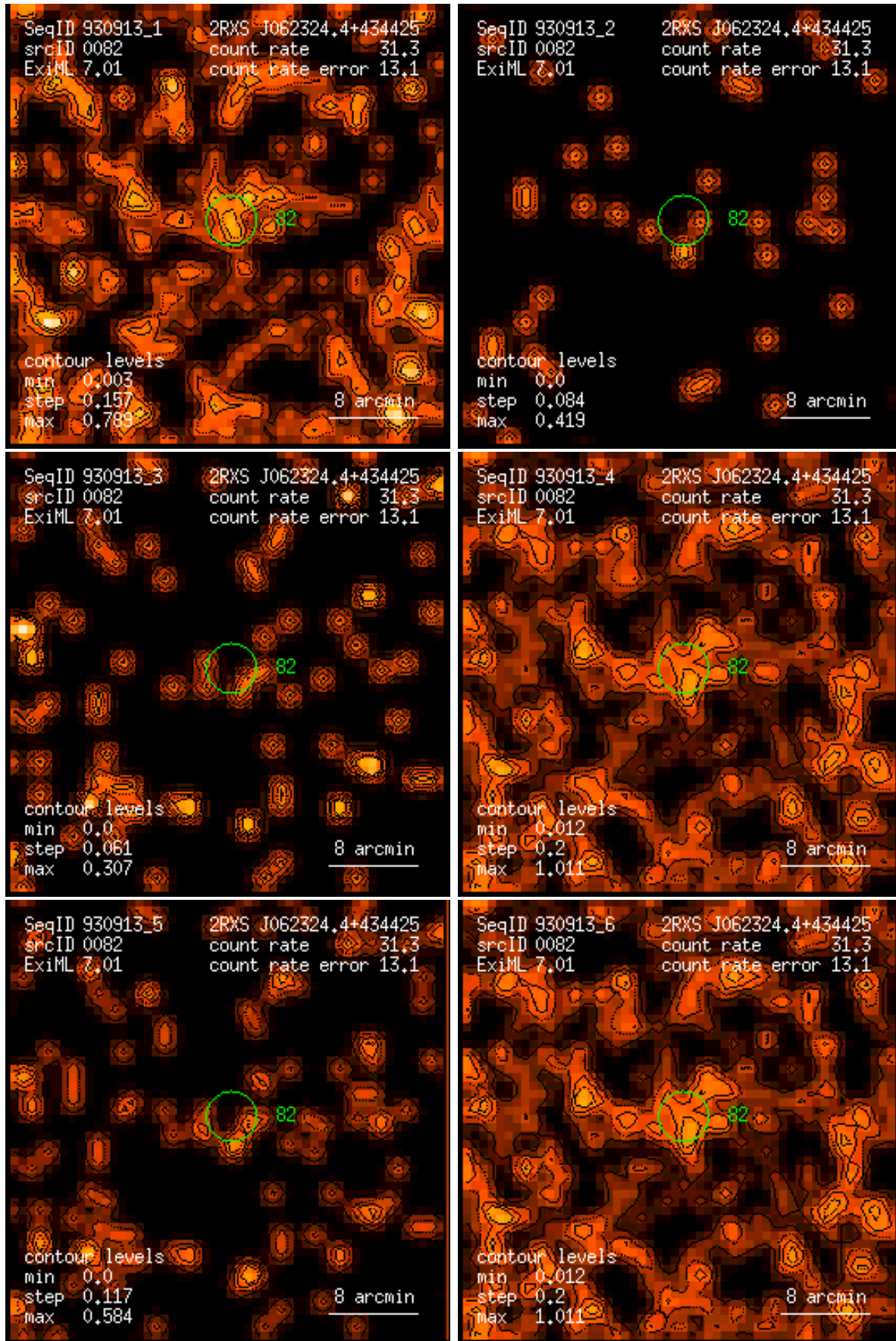
Figure 82: RASS 930913: detection 0082: band rate images, Gaussian filter: (1) PSPC channels 11 – 41, (2) 52 – 90, (3) 91 – 201, (4) 11 – 235, (5) 52 – 201, (6) 11 – 201. Broad band rates in counts/ks. Band rate contour levels in counts/ks/arcmin 2 .
