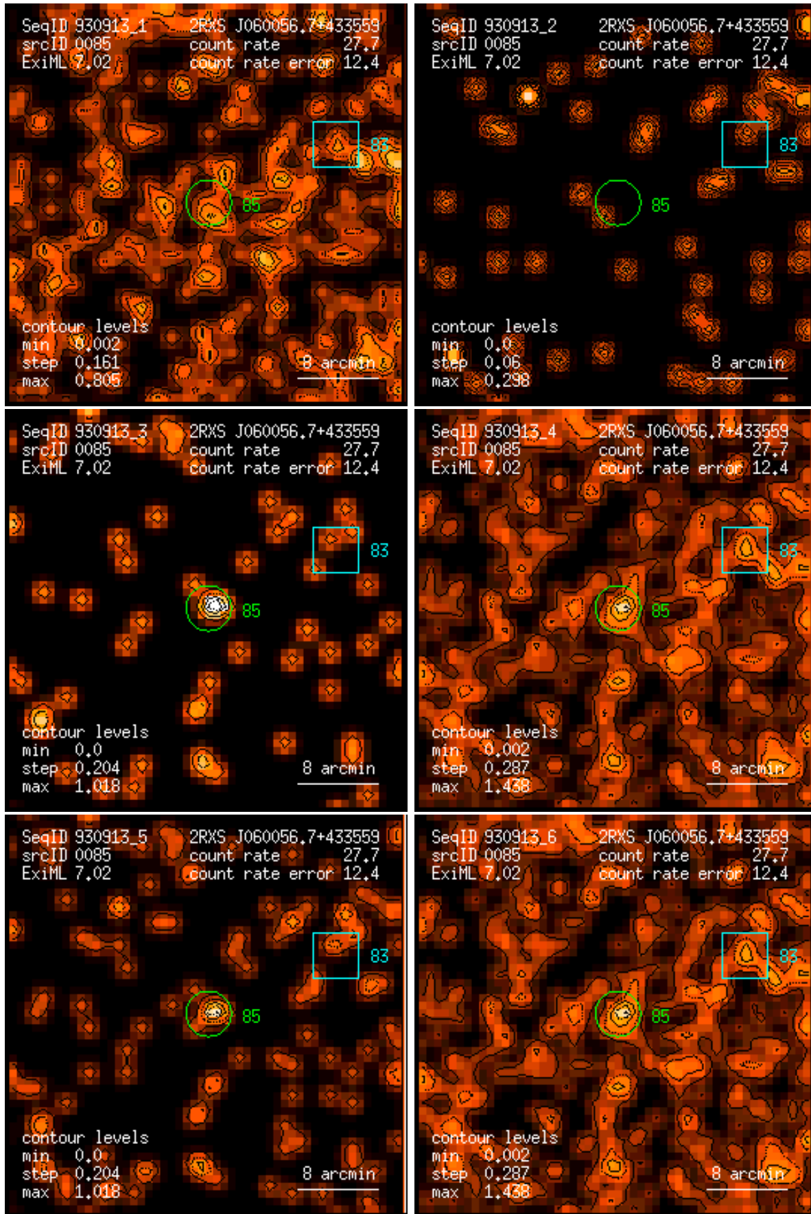
Figure 85: RASS 930913: detection 0085: band rate images, Gaussian filter: (1) PSPC channels 11 – 41, (2) 52 – 90, (3) 91 – 201, (4) 11 – 235, (5) 52 – 201, (6) 11 – 201. Broad band rates in counts/ks. Band rate contour levels in counts/ks/arcmin 2 .
