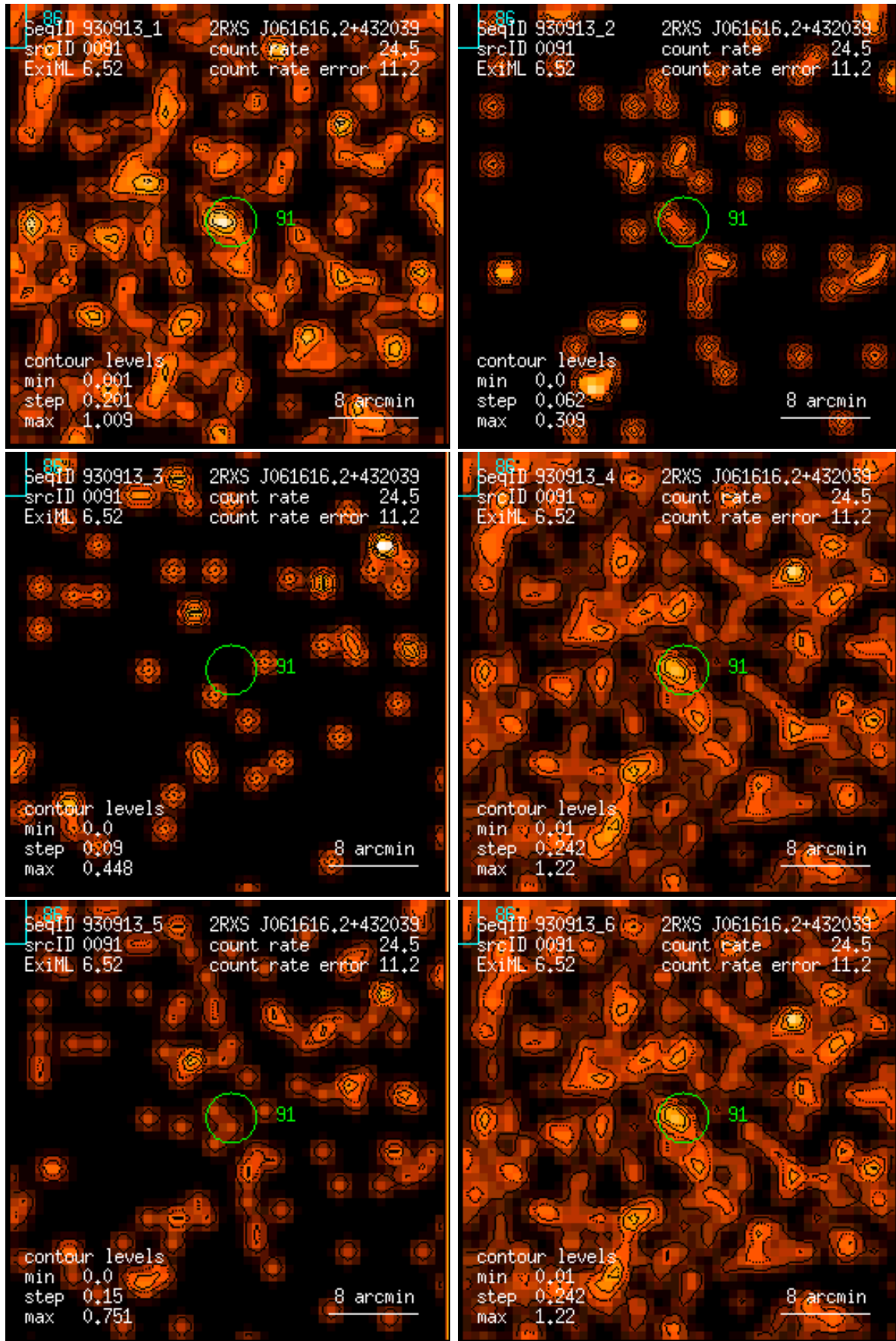
Figure 91: RASS 930913: detection 0091: band rate images, Gaussian filter: (1) PSPC channels 11 – 41, (2) 52 – 90, (3) 91 – 201, (4) 11 – 235, (5) 52 – 201, (6) 11 – 201. Broad band rates in counts/ks. Band rate contour levels in counts/ks/arcmin 2 .
