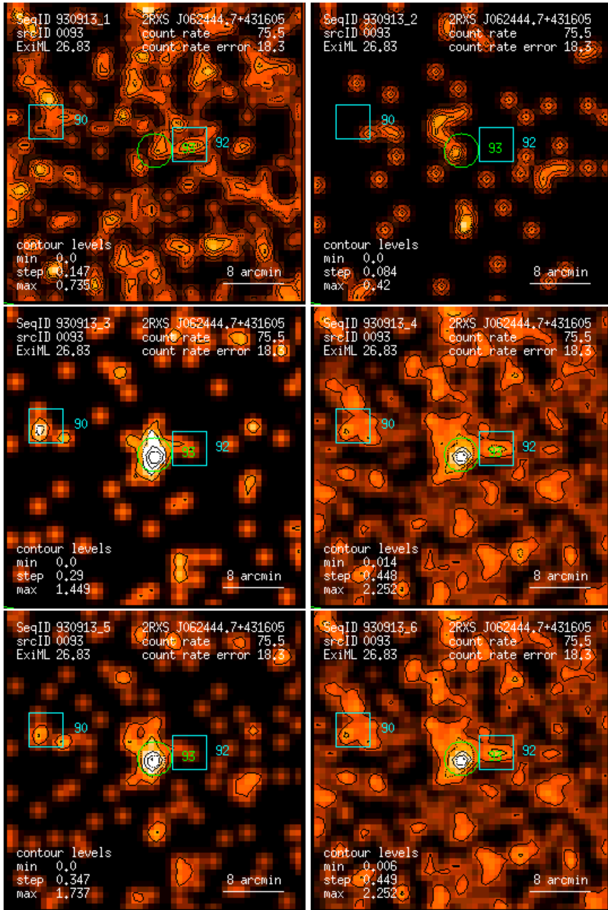
Figure 93: RASS 930913: detection 0093: band rate images, Gaussian filter: (1) PSPC channels 11 – 41, (2) 52 – 90, (3) 91 – 201, (4) 11 – 235, (5) 52 – 201, (6) 11 – 201. Broad band rates in counts/ks. Band rate contour levels in counts/ks/arcmin 2 .
