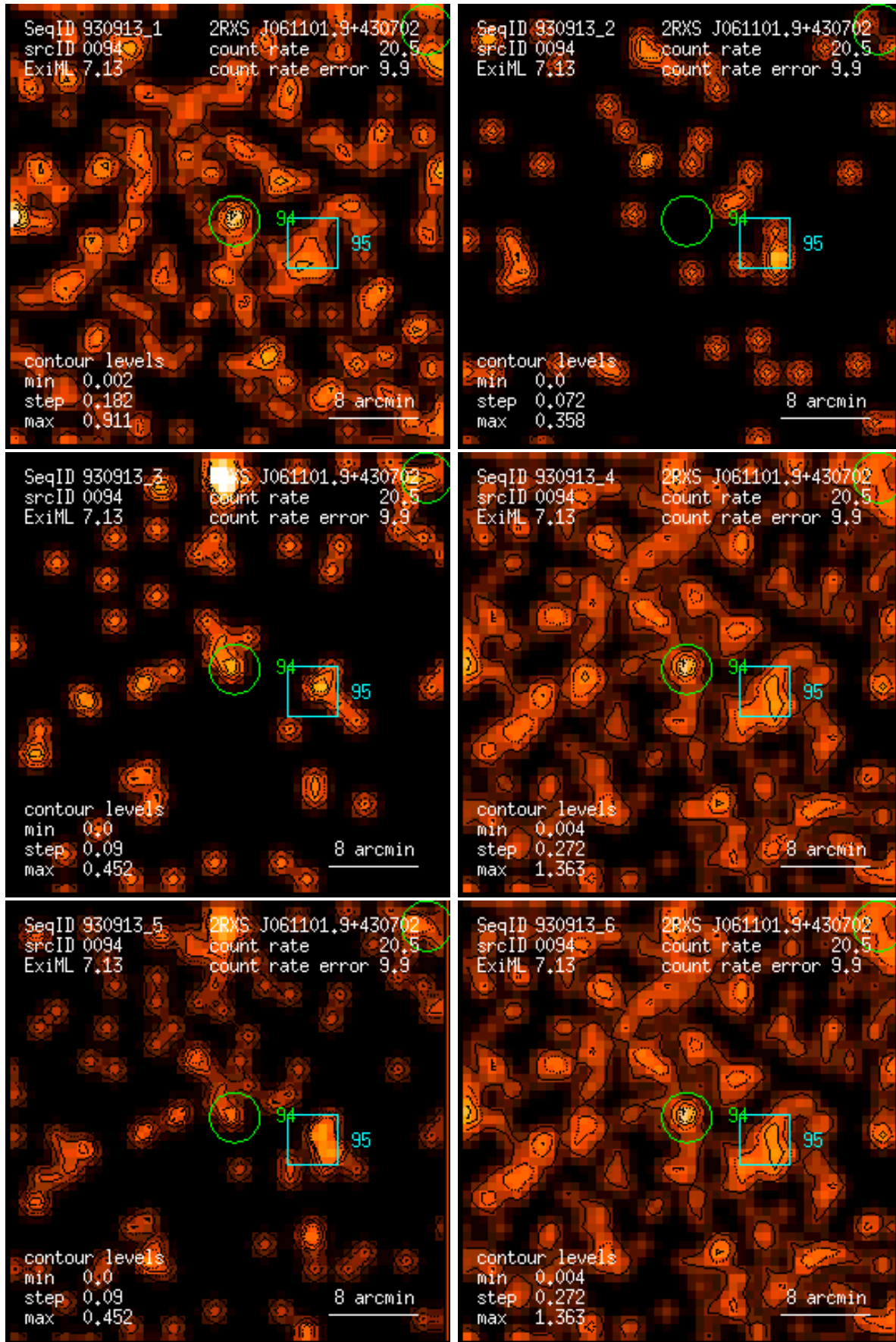
Figure 94: RASS 930913: detection 0094: band rate images, Gaussian filter: (1) PSPC channels 11 – 41, (2) 52 – 90, (3) 91 – 201, (4) 11 – 235, (5) 52 – 201, (6) 11 – 201. Broad band rates in counts/ks. Band rate contour levels in counts/ks/arcmin 2 .
