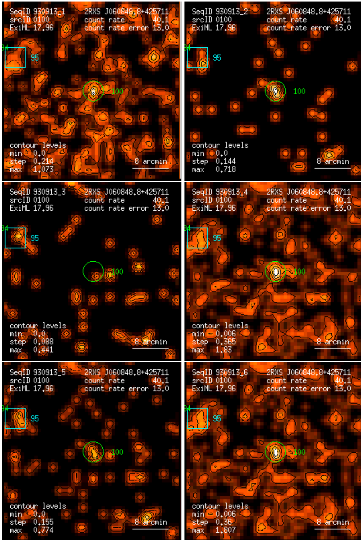
Figure 100: RASS 930913: detection 0100: band rate images, Gaussian filter: (1) PSPC channels 11 – 41, (2) 52 – 90, (3) 91 – 201, (4) 11 – 235, (5) 52 – 201, (6) 11 – 201. Broad band rates in counts/ks. Band rate contour levels in counts/ks/arcmin 2 .
