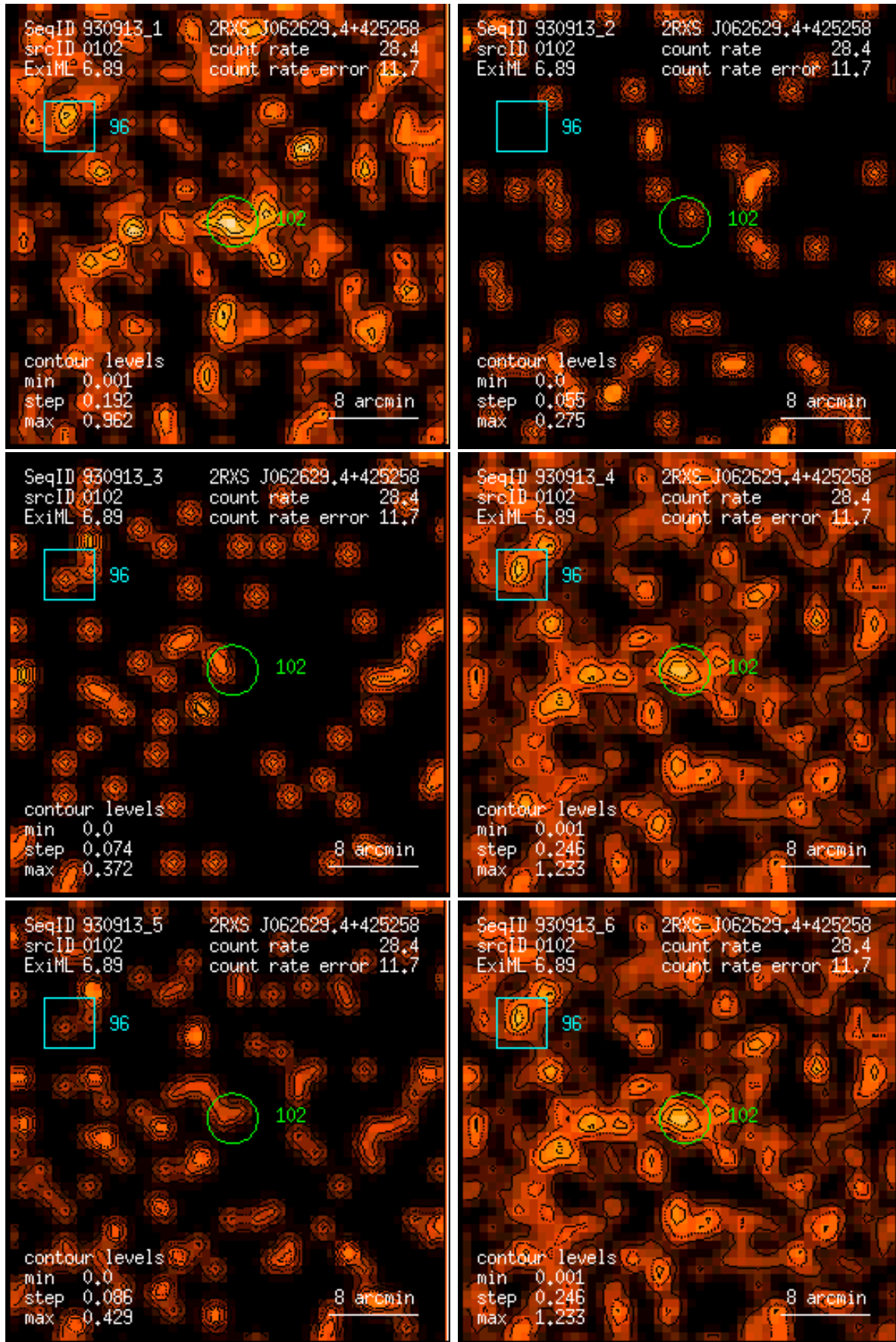
Figure 102: RASS 930913: detection 0102: band rate images, Gaussian filter: (1) PSPC channels 11 – 41, (2) 52 – 90, (3) 91 – 201, (4) 11 – 235, (5) 52 – 201, (6) 11 – 201. Broad band rates in counts/ks. Band rate contour levels in counts/ks/arcmin 2 .
