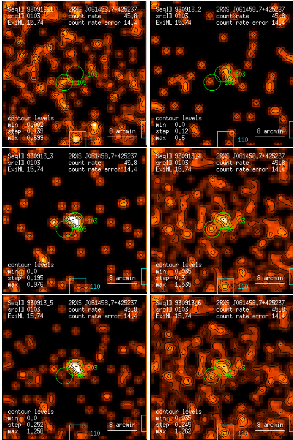
Figure 103: RASS 930913: detection 0103: band rate images, Gaussian filter: (1) PSPC channels 11 – 41, (2) 52 – 90, (3) 91 – 201, (4) 11 – 235, (5) 52 – 201, (6) 11 – 201. Broad band rates in counts/ks. Band rate contour levels in counts/ks/arcmin 2 .
