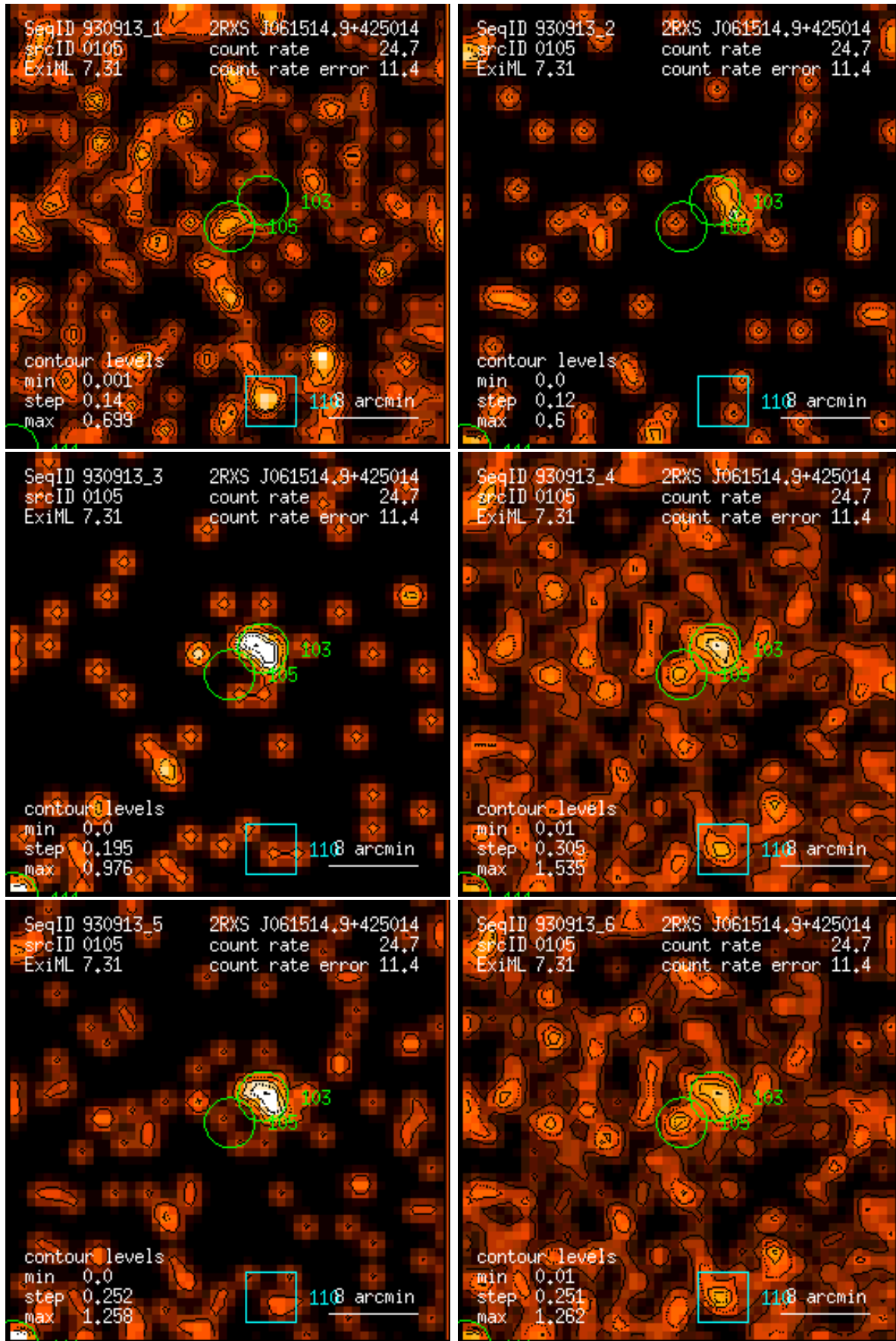
Figure 105: RASS 930913: detection 0105: band rate images, Gaussian filter: (1) PSPC channels 11 – 41, (2) 52 – 90, (3) 91 – 201, (4) 11 – 235, (5) 52 – 201, (6) 11 – 201. Broad band rates in counts/ks. Band rate contour levels in counts/ks/arcmin 2 .
