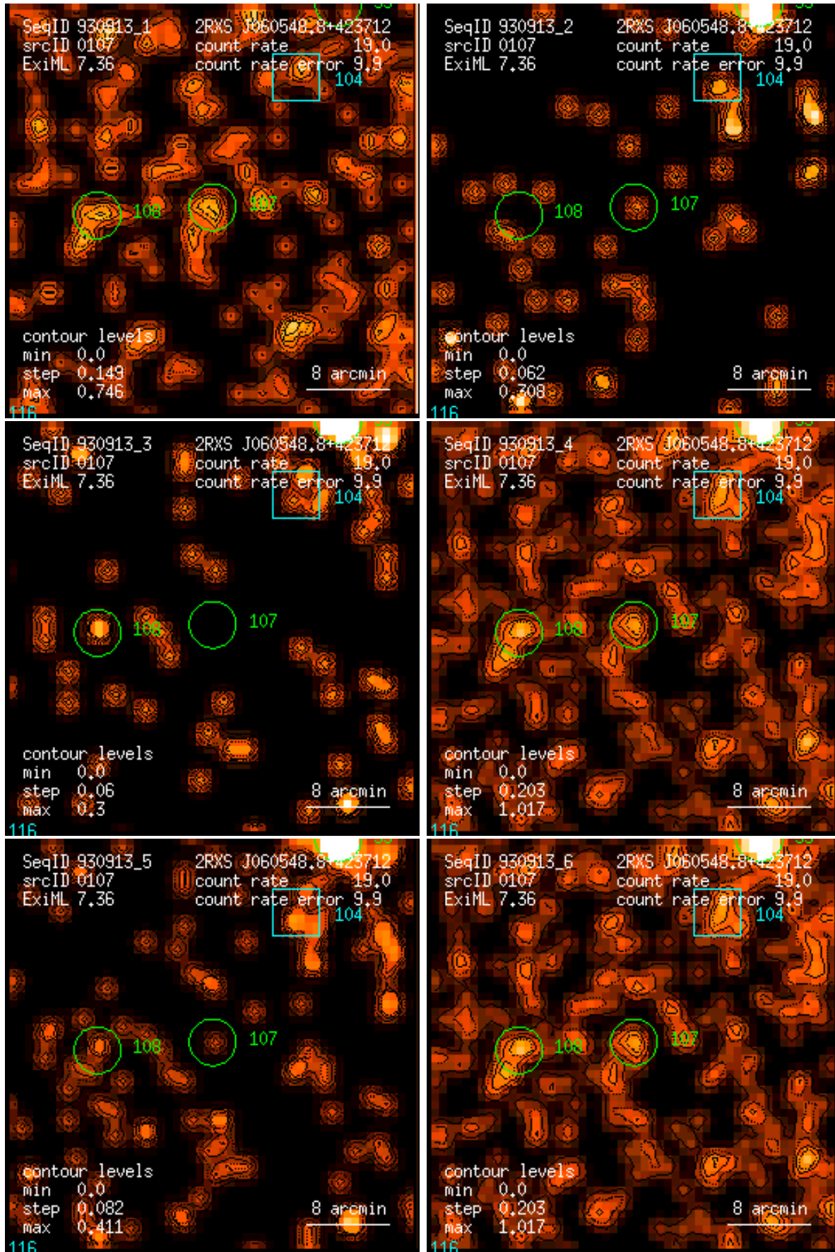
Figure 107: RASS 930913: detection 0107: band rate images, Gaussian filter: (1) PSPC channels 11 – 41, (2) 52 – 90, (3) 91 – 201, (4) 11 – 235, (5) 52 – 201, (6) 11 – 201. Broad band rates in counts/ks. Band rate contour levels in counts/ks/arcmin 2 .
