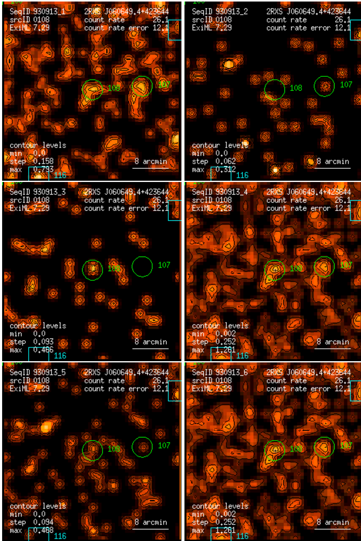
Figure 108: RASS 930913: detection 0108: band rate images, Gaussian filter: (1) PSPC channels 11 – 41, (2) 52 – 90, (3) 91 – 201, (4) 11 – 235, (5) 52 – 201, (6) 11 – 201. Broad band rates in counts/ks. Band rate contour levels in counts/ks/arcmin 2 .
