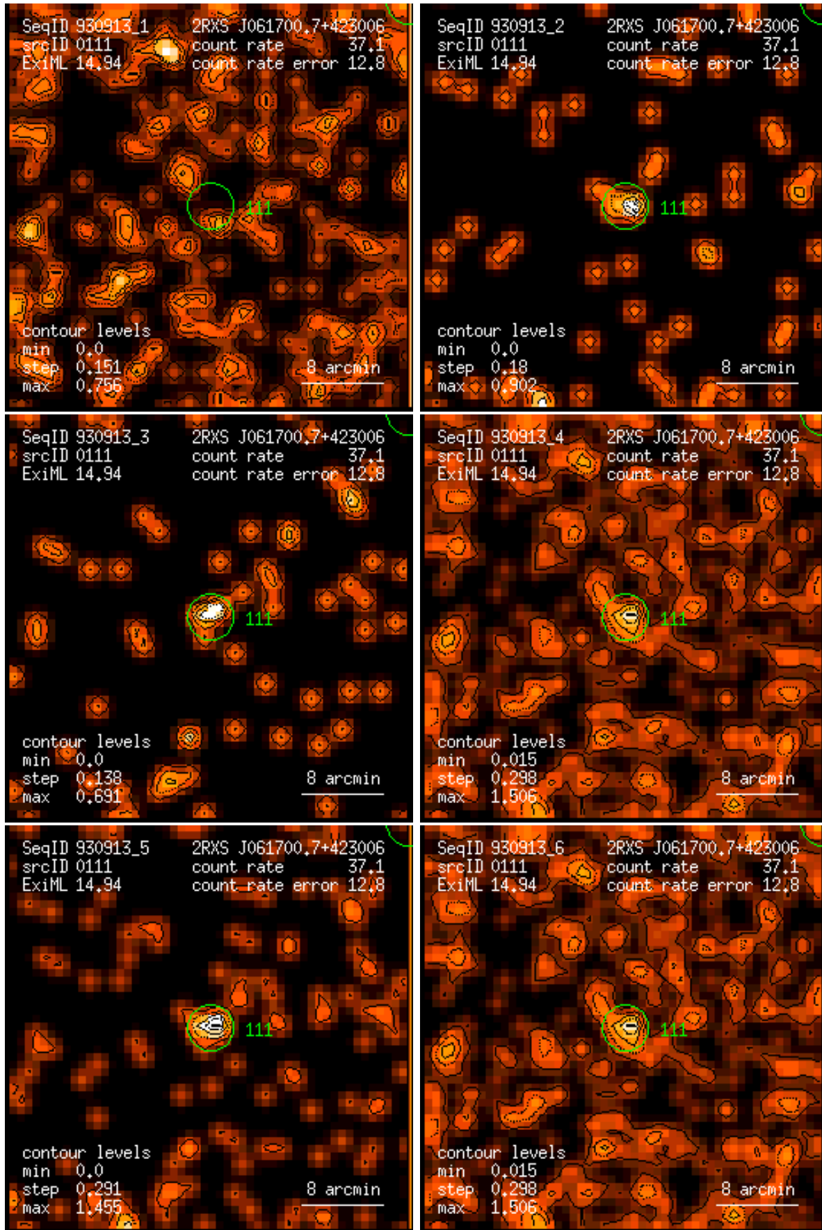
Figure 111: RASS 930913: detection 0111: band rate images, Gaussian filter: (1) PSPC channels 11 – 41, (2) 52 – 90, (3) 91 – 201, (4) 11 – 235, (5) 52 – 201, (6) 11 – 201. Broad band rates in counts/ks. Band rate contour levels in counts/ks/arcmin 2 .
