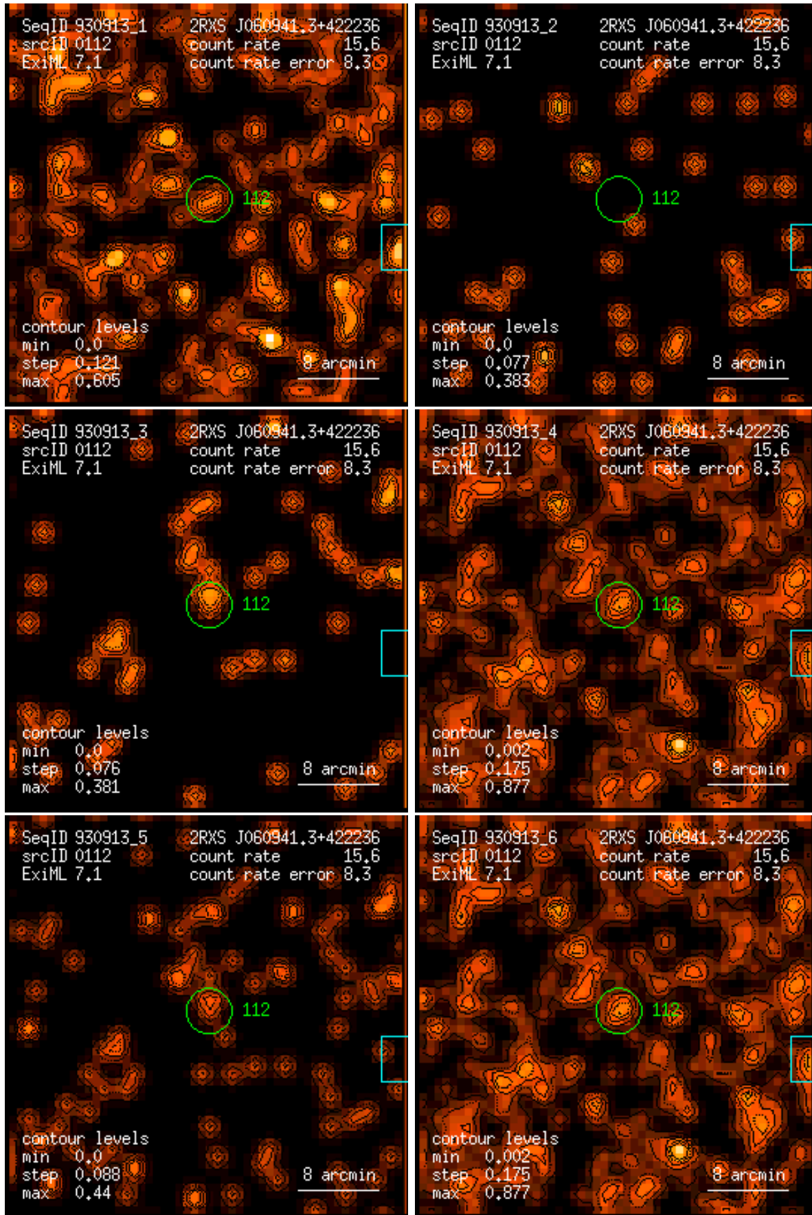
Figure 112: RASS 930913: detection 0112: band rate images, Gaussian filter: (1) PSPC channels 11 – 41, (2) 52 – 90, (3) 91 – 201, (4) 11 – 235, (5) 52 – 201, (6) 11 – 201. Broad band rates in counts/ks. Band rate contour levels in counts/ks/arcmin 2 .
