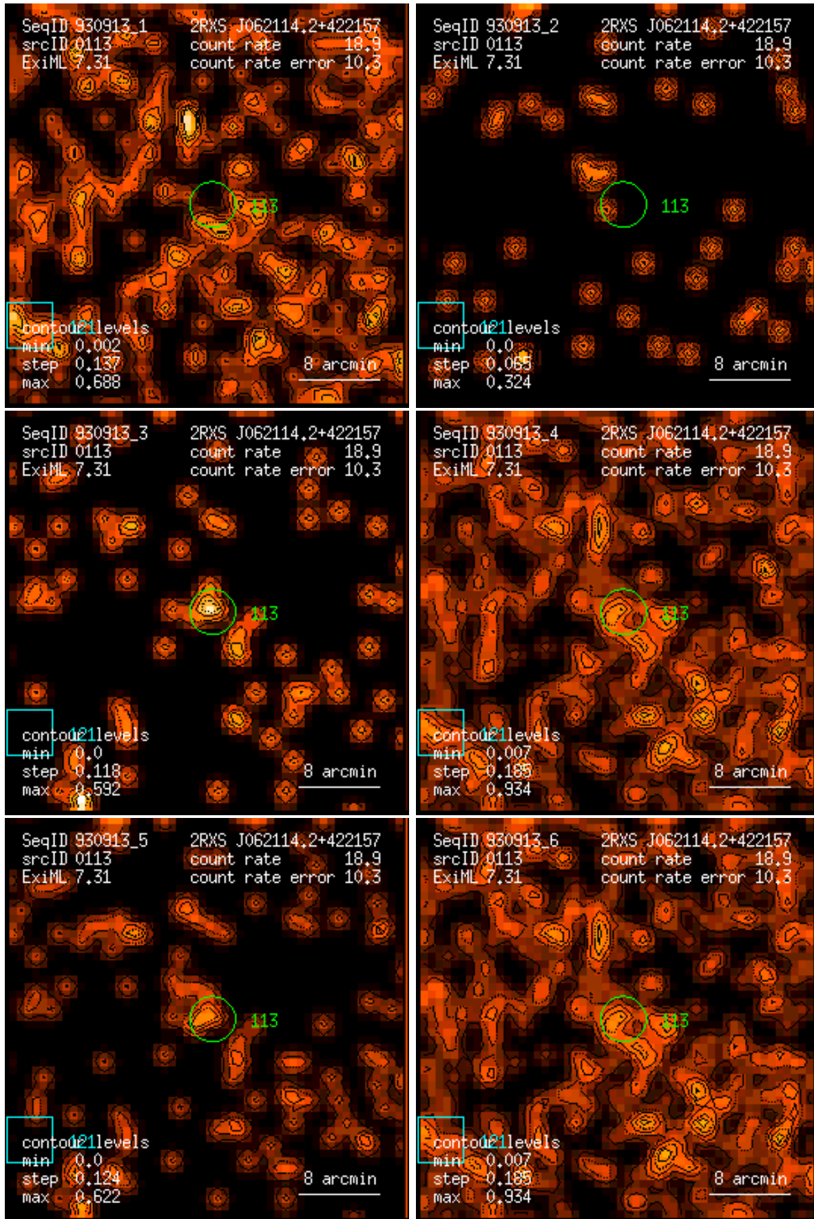
Figure 113: RASS 930913: detection 0113: band rate images, Gaussian filter: (1) PSPC channels 11 – 41, (2) 52 – 90, (3) 91 – 201, (4) 11 – 235, (5) 52 – 201, (6) 11 – 201. Broad band rates in counts/ks. Band rate contour levels in counts/ks/arcmin 2 .
