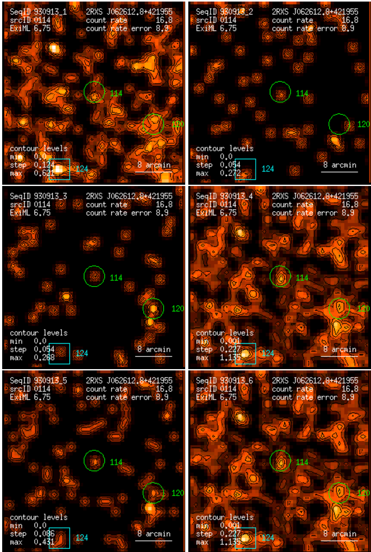
Figure 114: RASS 930913: detection 0114: band rate images, Gaussian filter: (1) PSPC channels 11 – 41, (2) 52 – 90, (3) 91 – 201, (4) 11 – 235, (5) 52 – 201, (6) 11 – 201. Broad band rates in counts/ks. Band rate contour levels in counts/ks/arcmin 2 .
