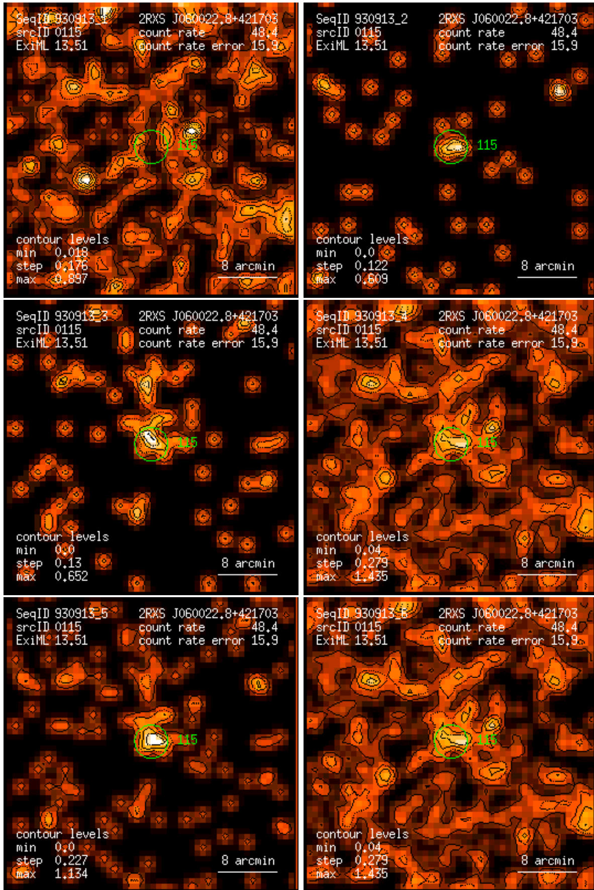
Figure 115: RASS 930913: detection 0115: band rate images, Gaussian filter: (1) PSPC channels 11 – 41, (2) 52 – 90, (3) 91 – 201, (4) 11 – 235, (5) 52 – 201, (6) 11 – 201. Broad band rates in counts/ks. Band rate contour levels in counts/ks/arcmin 2 .
