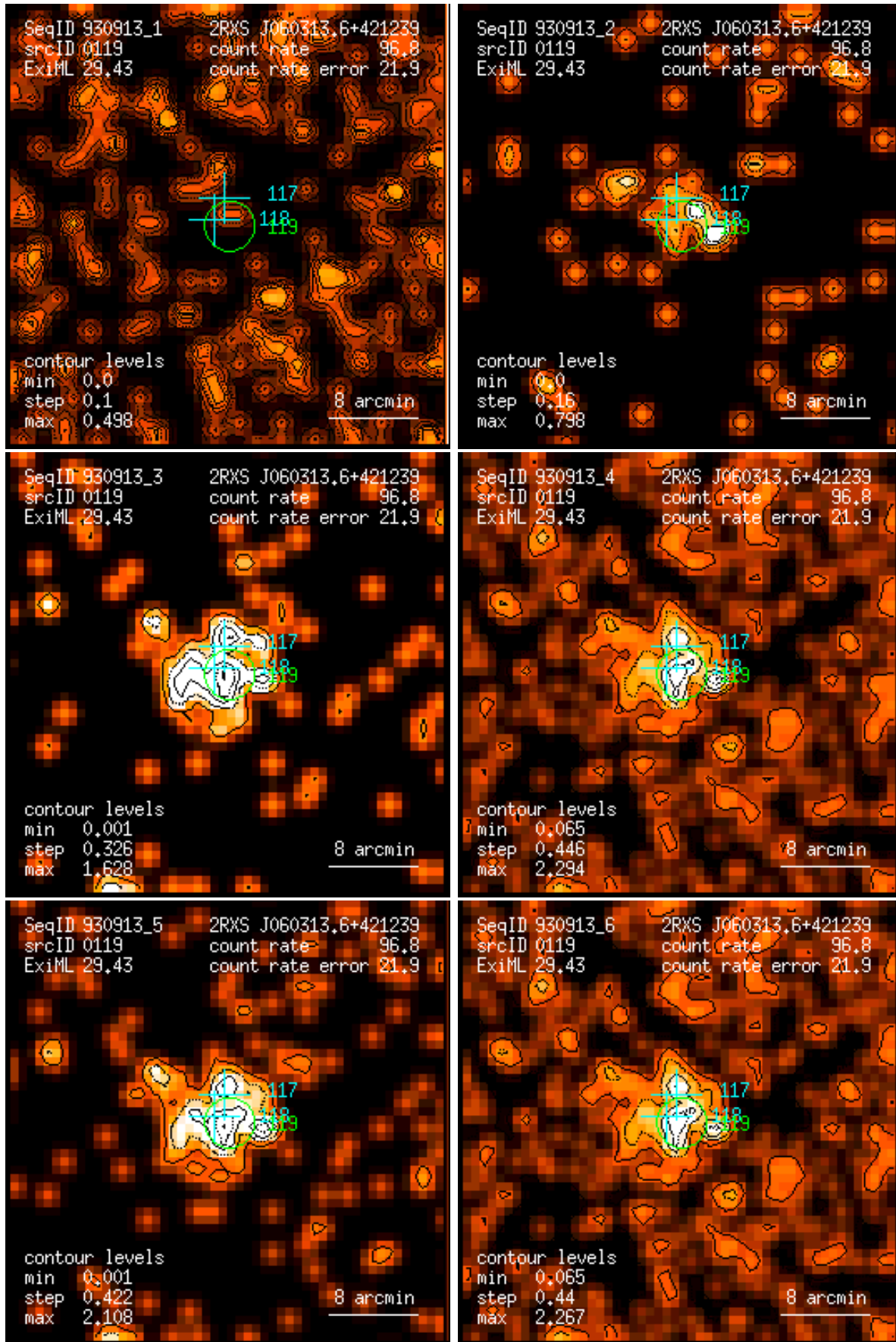
Figure 119: RASS 930913: detection 0119: band rate images, Gaussian filter: (1) PSPC channels 11 – 41, (2) 52 – 90, (3) 91 – 201, (4) 11 – 235, (5) 52 – 201, (6) 11 – 201. Broad band rates in counts/ks. Band rate contour levels in counts/ks/arcmin 2 .
