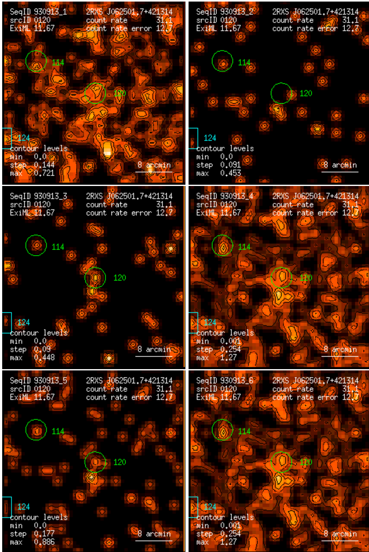
Figure 120: RASS 930913: detection 0120: band rate images, Gaussian filter: (1) PSPC channels 11 – 41, (2) 52 – 90, (3) 91 – 201, (4) 11 – 235, (5) 52 – 201, (6) 11 – 201. Broad band rates in counts/ks. Band rate contour levels in counts/ks/arcmin 2 .
