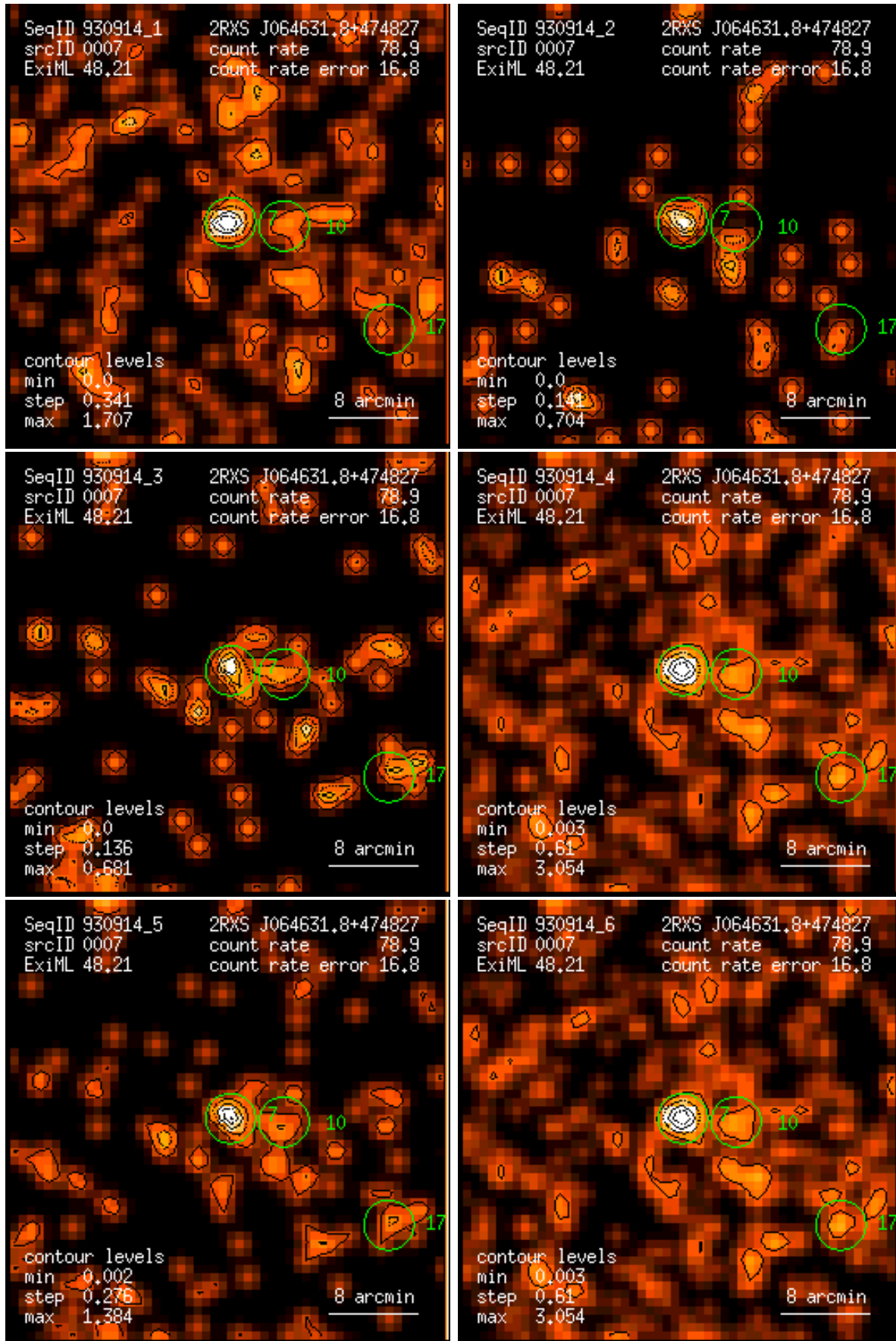
Figure 7: RASS 930914: detection 0007: band rate images, Gaussian filter: (1) PSPC channels 11 – 41, (2) 52 – 90, (3) 91 – 201, (4) 11 – 235, (5) 52 – 201, (6) 11 – 201. Broad band rates in counts/ks. Band rate contour levels in counts/ks/arcmin 2 .
